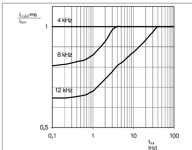
Fig. 11: Normalized output current vs. output frequency
