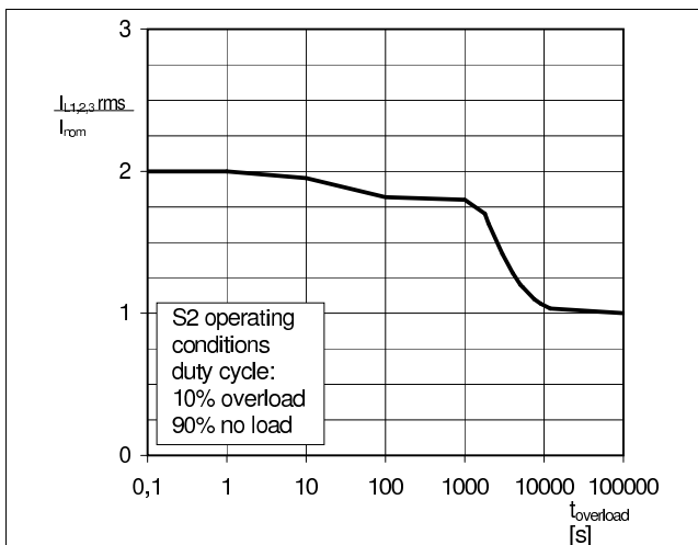
Fig. 5: Overload capability
