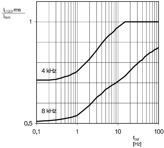
Fig. 9: Normalized output current vs. output frequency
