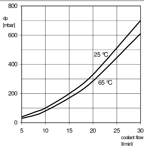
Fig. 7: Pressure drop characteristic
