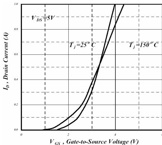
Fig 11. Transfer Characteristics
