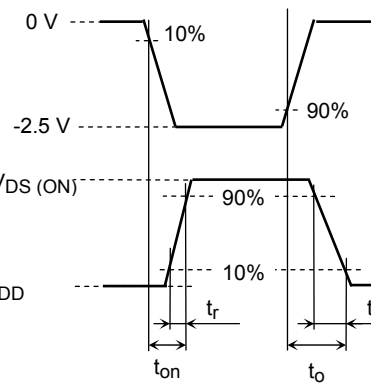
(c) V_{OUT}
