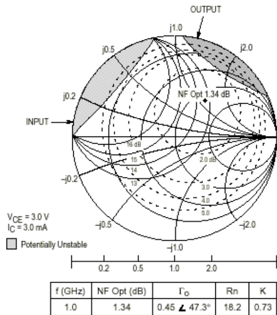
Fig. 21 Constant Gain & Noise Figure Coutsours
