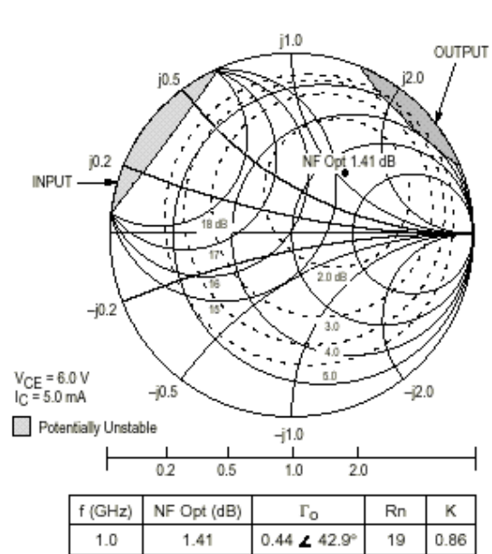
Fig. 22 Constant Gain & Noise Figure Coutsours
