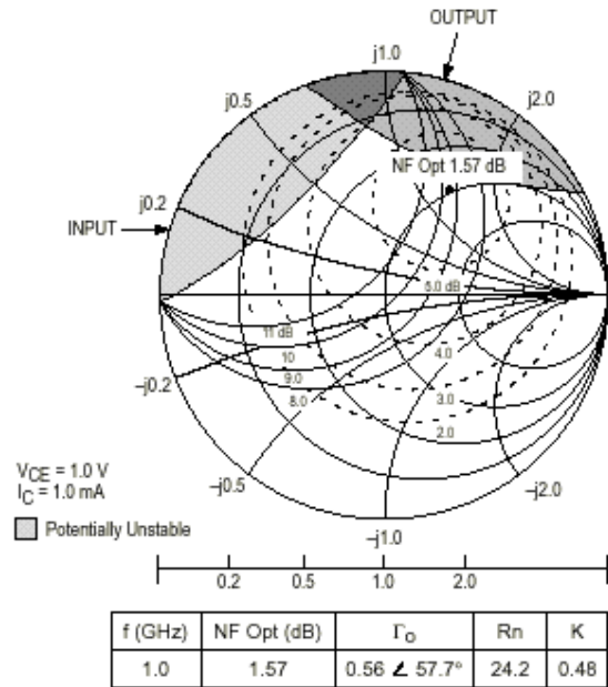
Fig. 19 Constant Gain & Noise Figure Coutsours
