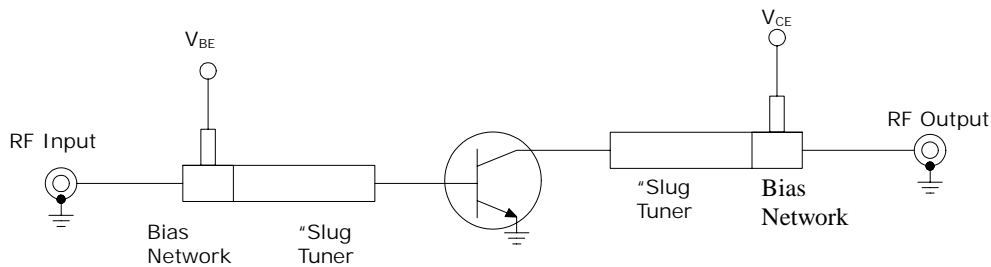
Fig. 5 Functional circuit schematic
