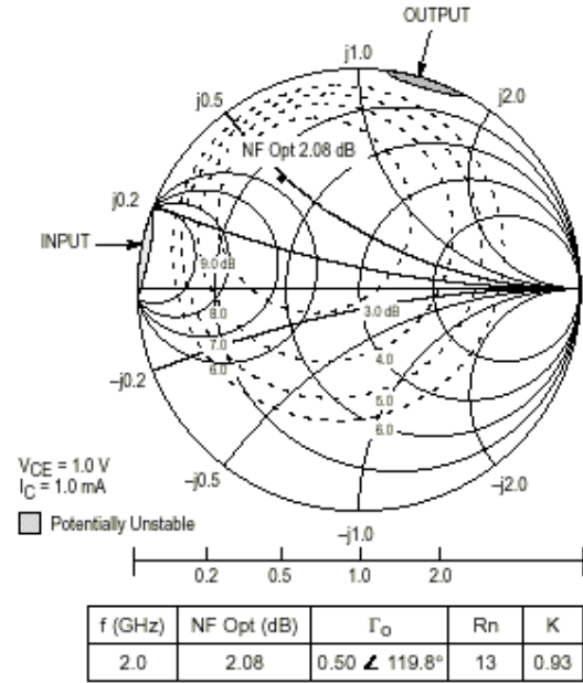
Fig. 20 Constant Gain & Noise Figure Coutsours
