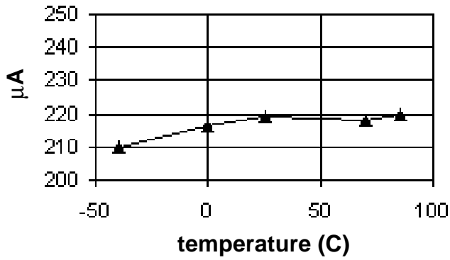
Icc vs. Temperature
