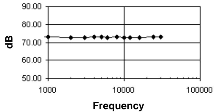
Signal to Noise Ratio
