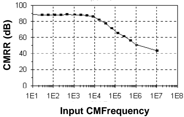
Input CMRR, Vcc = 5V
