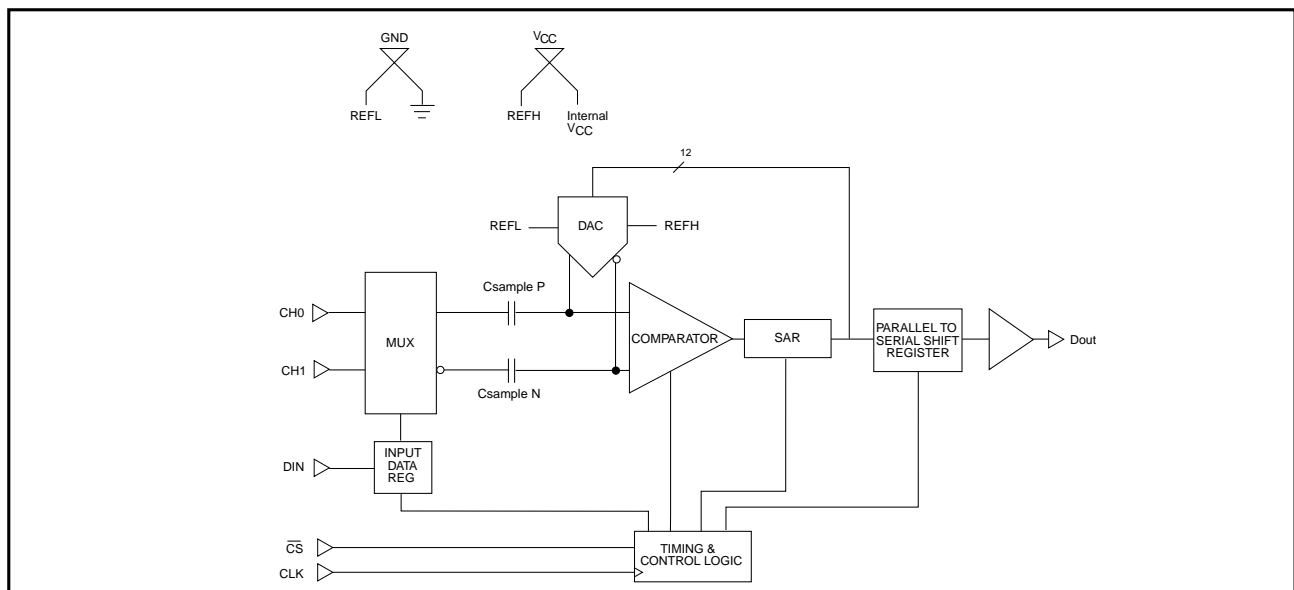
SP8538 Block Diagram
