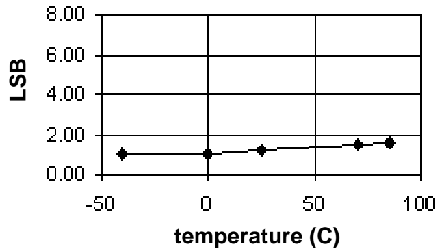
Gain Error vs. Temperature
