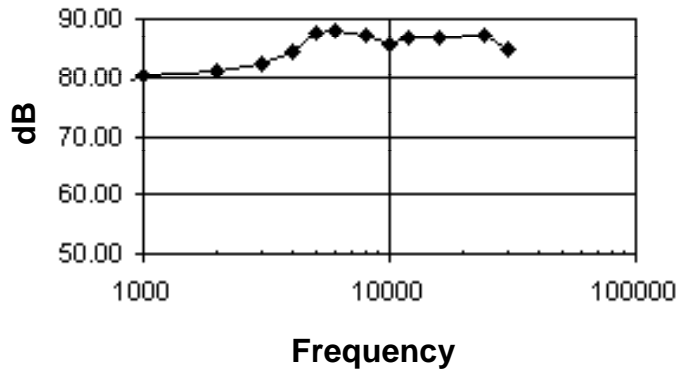
Spurious Free Dynamic Range
