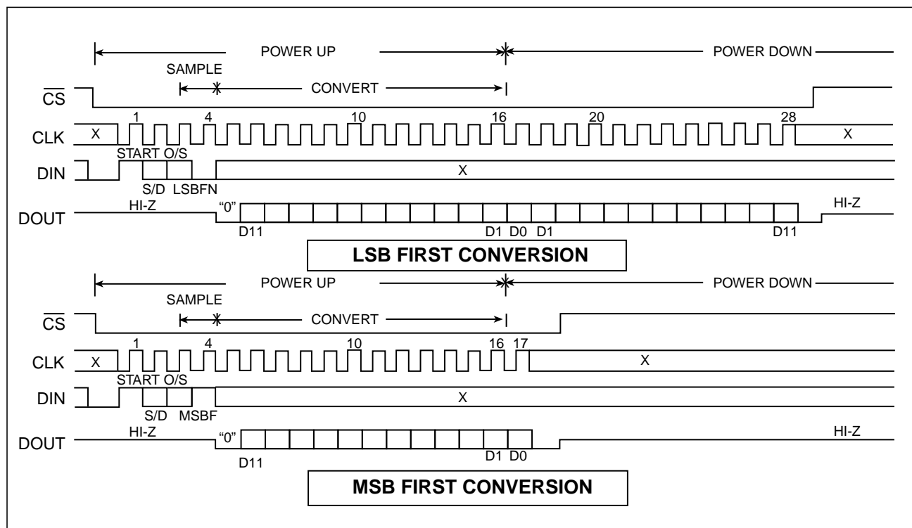
SP8538 Timing Diagram
