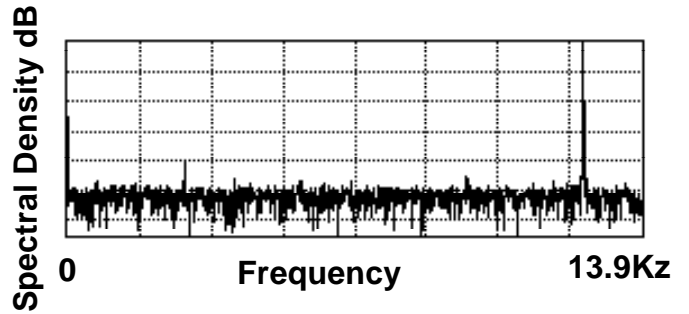
FFT 20 dB/div
