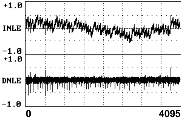
Vcc = 5.00V
