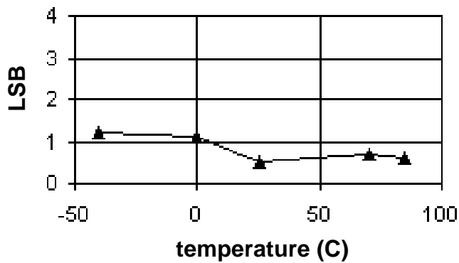
Offset vs. Temperature
