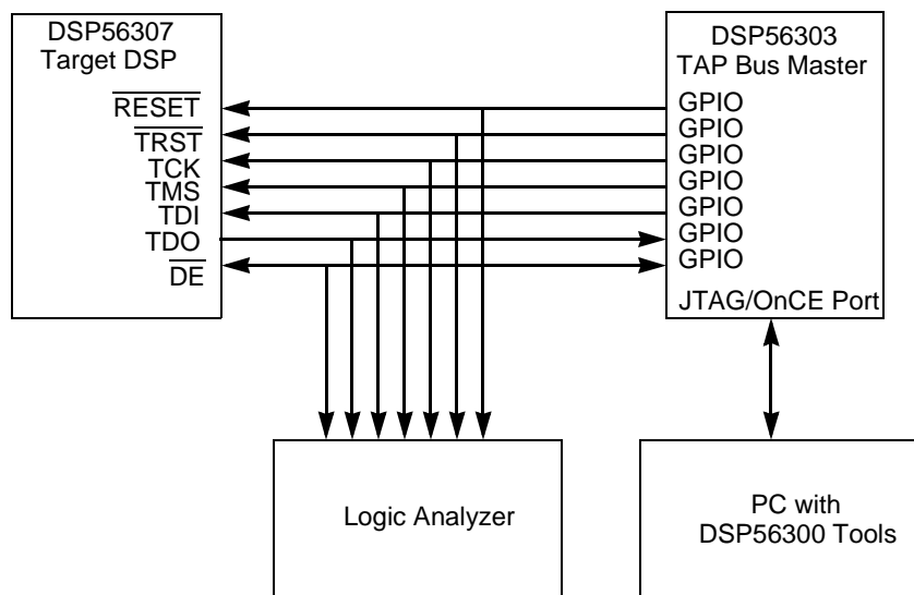
Figure 5. Test Setup
