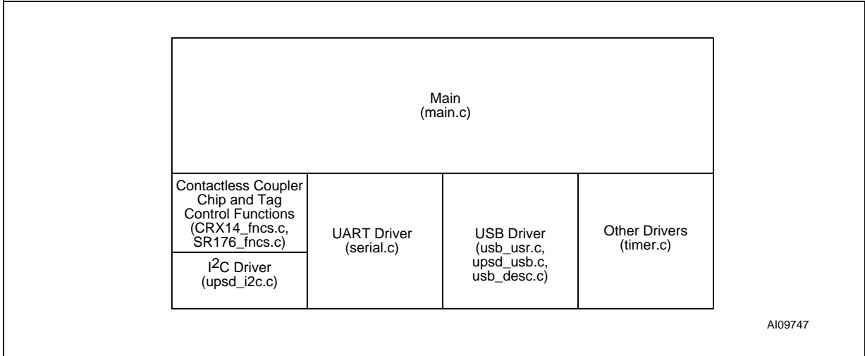
Figure 7. Block Diagram
