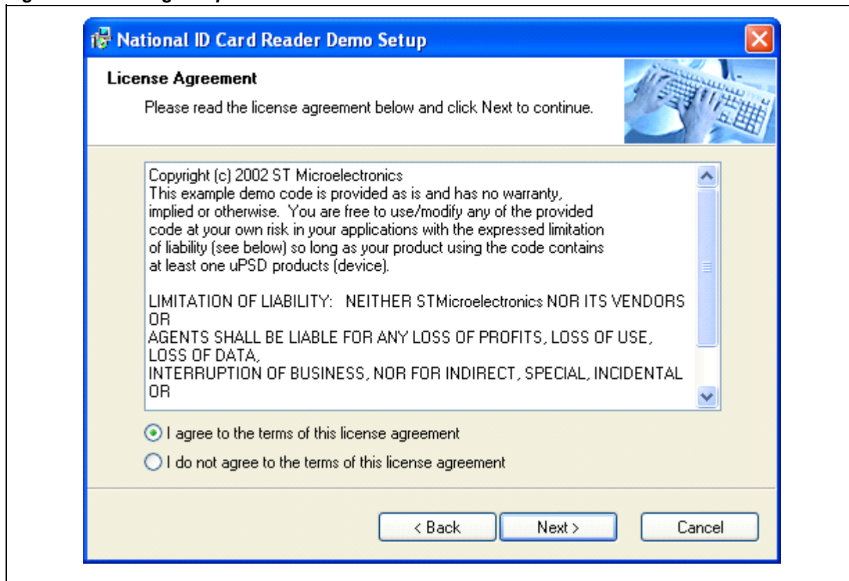
Figure 12. Running setup.exe
