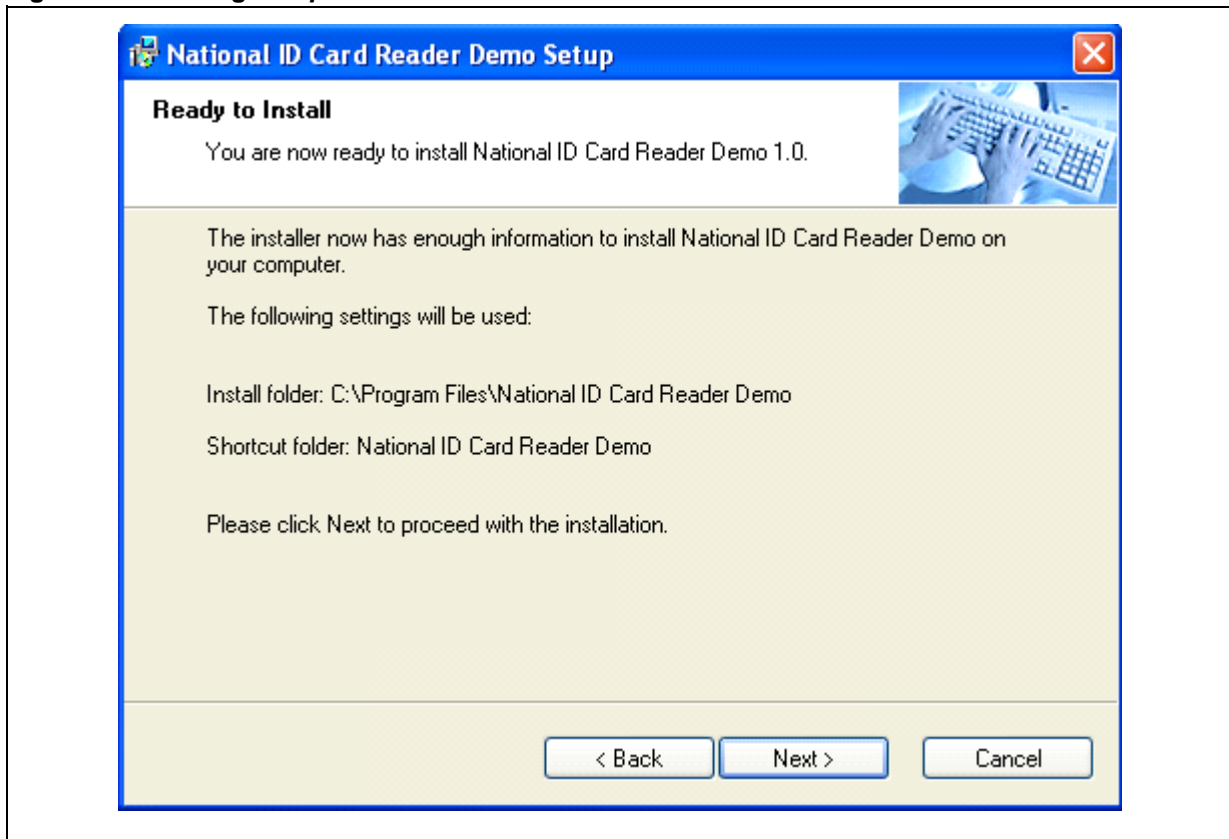
Figure 13. Running setup.exe
