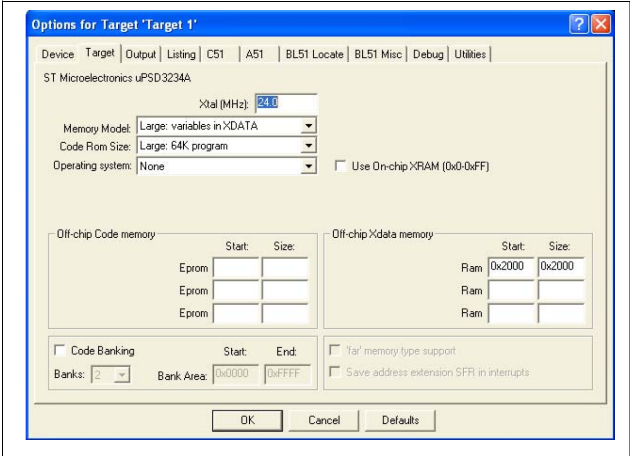
Figure 16. Keil Compiler Settings
