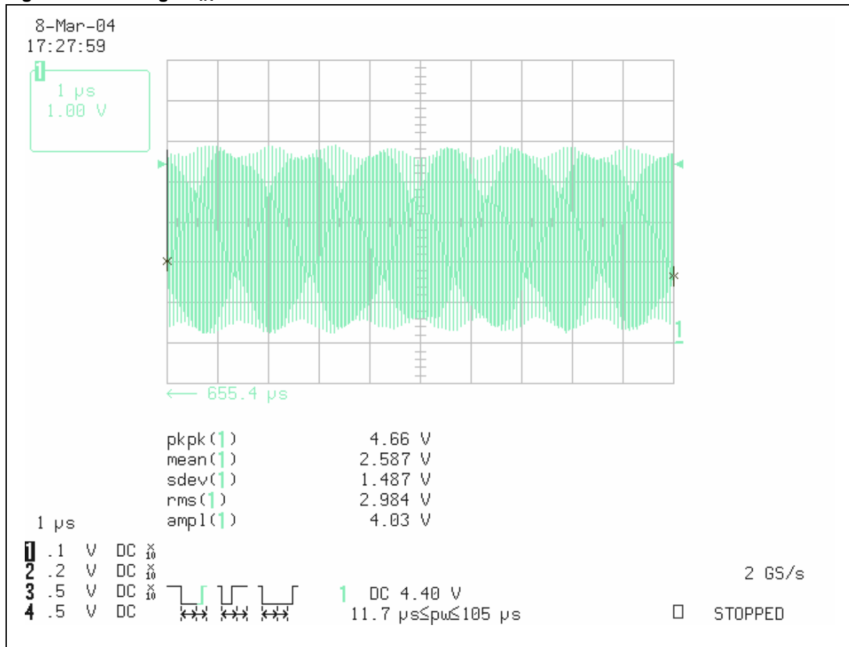
Figure 6. Checking RF IN
