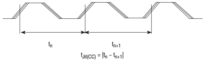
Figure 6. Cycle-to-Cycle Jitter
