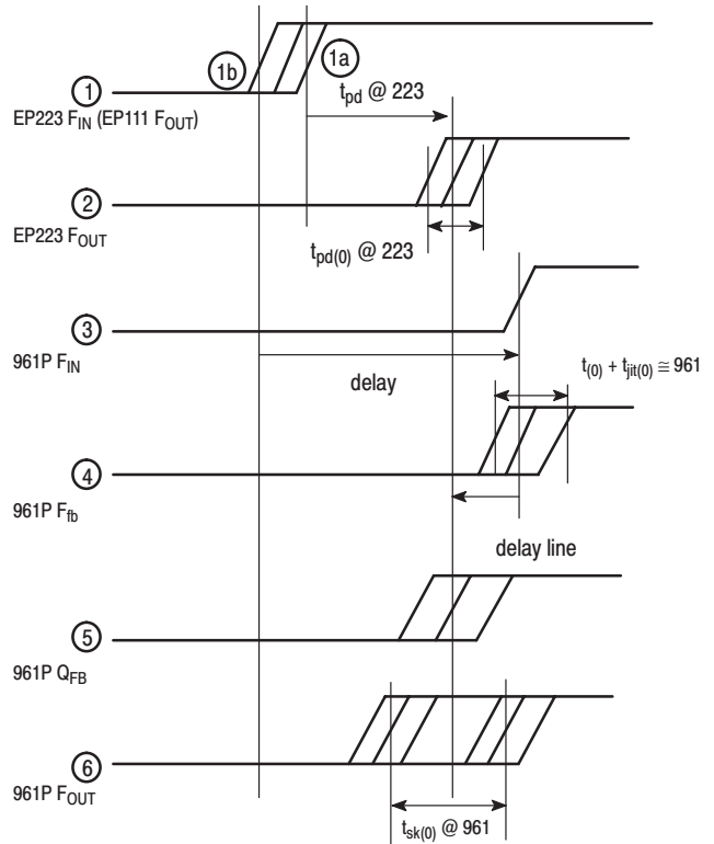
Figure 14. Example Clock Tree Analysis with Jitter and Skew
