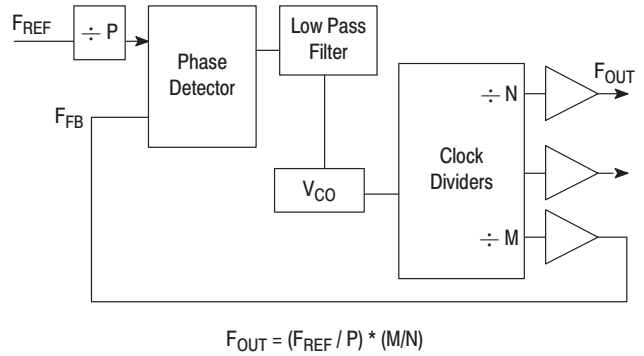
Figure 4. PLL Based Clock Driver
