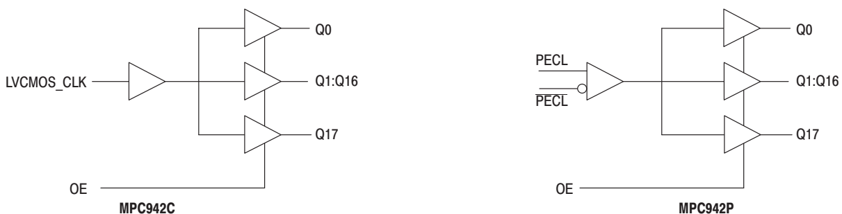
Figure 2. Fanout Buffer
