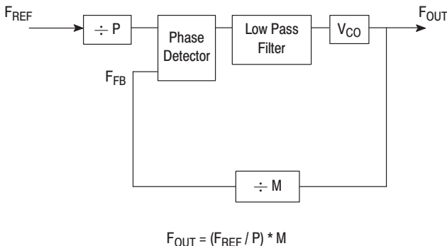
Figure 3. Basic PLL
