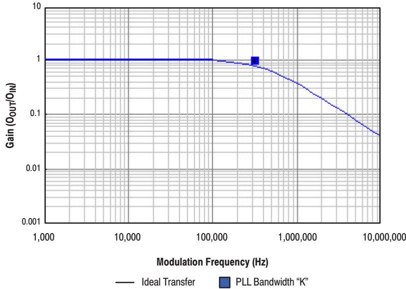
Figure 11. PLL Bandwidth
