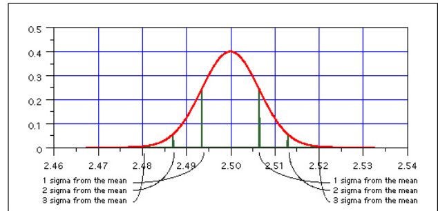
Figure 9. Classic Gaussian Distribution Curve
