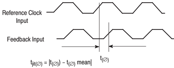
Figure 8. Phase Jitter
