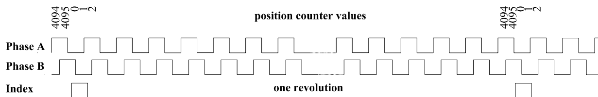
Figure 3-9. Quadrature Encoder output signals
