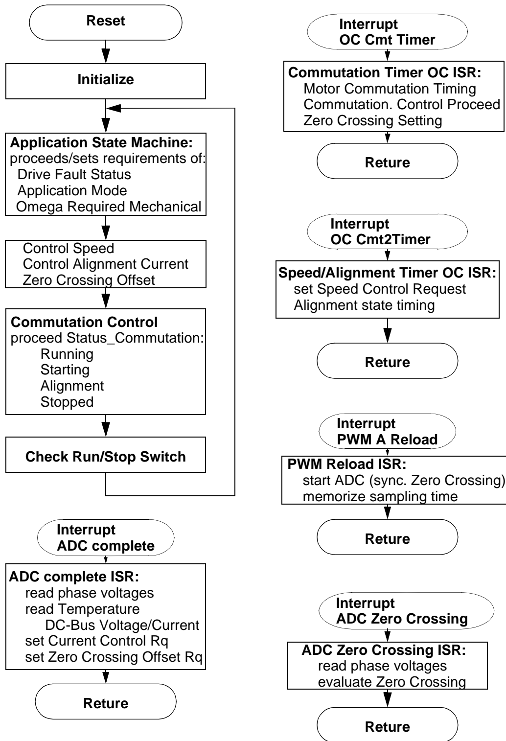
Figure 7-1. Main Software Flow Chart - Part 1
