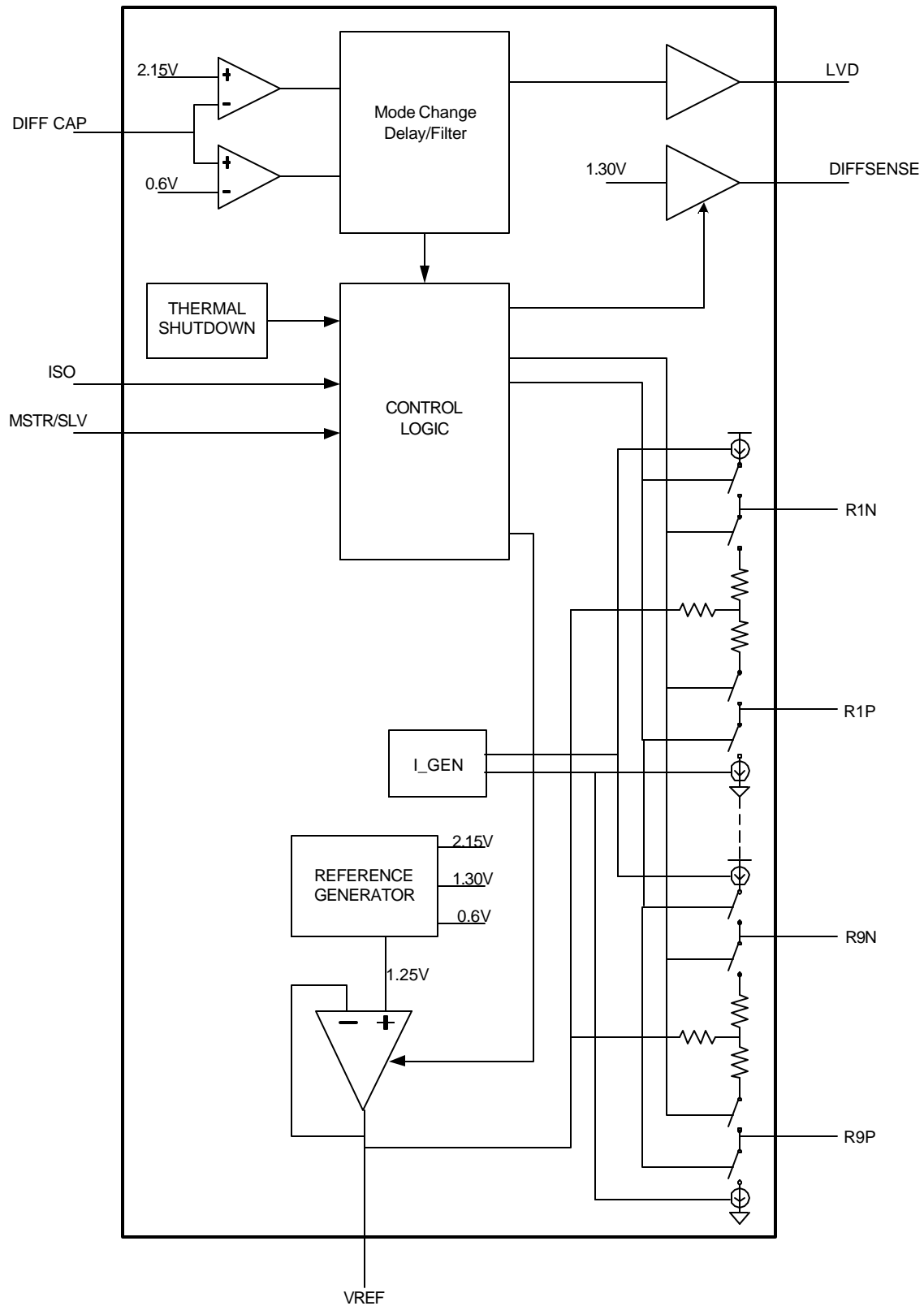
Figure 1. BLOCK DIAGRAM
