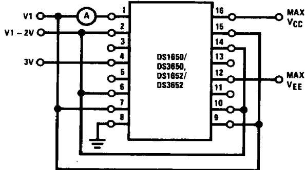
FIGURE 5. I_{IH}
