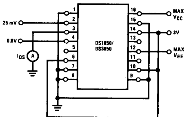
FIGURE 4. I_{OS}
