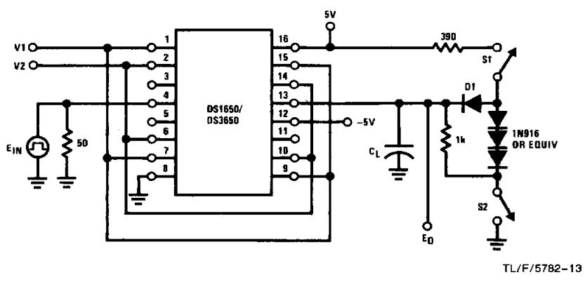
FIGURE 8. Receiver Propagation Delay t_{PLH(D)} and t_{PHL(D)}
