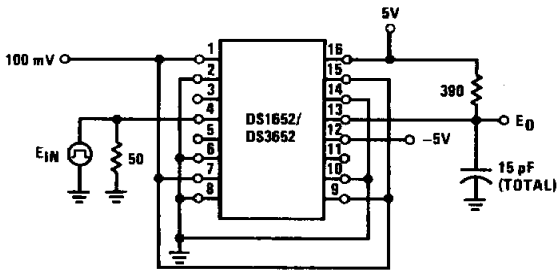
FIGURE 10. Strobe Propagation Delay t_{PLH(S)} and t_{PHL(S)}
