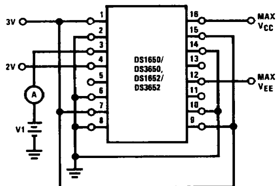
FIGURE 5. I_{IH}
