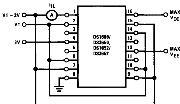
FIGURE 6. I_{iL}
