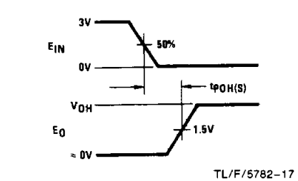
FIGURE 9. Strobe Propagation Delay t_{PLO(S)} , t_{POL(S)} , t_{PHO(S)} and t_{POH(S)}
