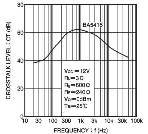
Fig. 21 Crosstalk vs. frequency (BA5416)
