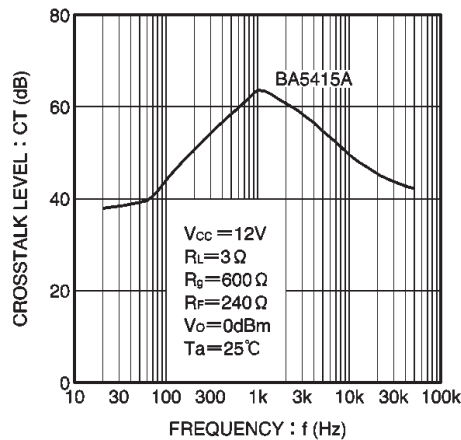
Fig. 20 Crosstalk vs. frequency (BA5415A)
