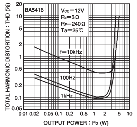
Fig. 15 Total harmonic distortion vs. output power (BA5416)
