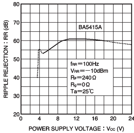
Fig. 23 Ripple rejection vs. power supply voltage (BA5415A)
