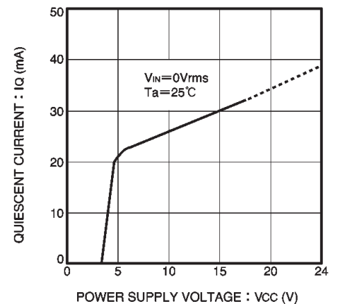
Fig. 12 Quiescent current vs. power supply voltage
