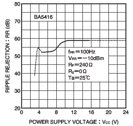
Fig. 24 Ripple rejection vs. power supply voltage (BA5416)
