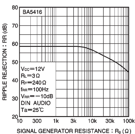
Fig. 28 Ripple rejection vs. signal source resistance (BA5416)
