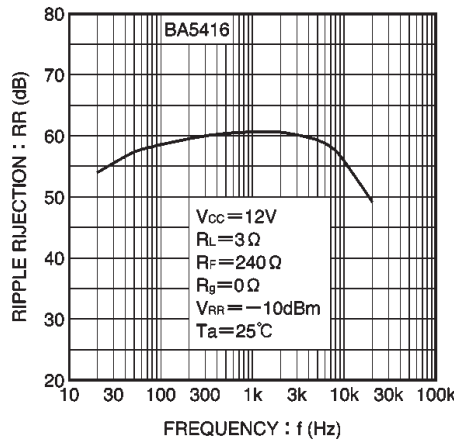
Fig. 26 Ripple rejection vs. frequency (BA5416)
