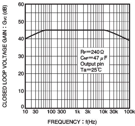
Fig. 13 Closed loop voltage gain vs. frequency
