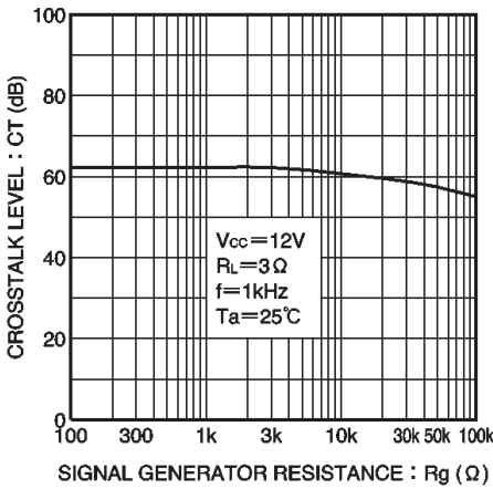
Fig. 22 Crosstalk vs. signal source resistance
