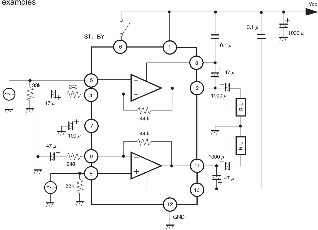
Fig. 2 OTL Application circuit example
