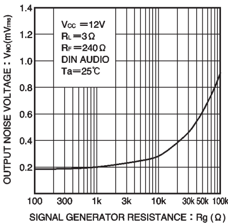
Fig. 19 Output noise voltage vs. signal source resistance
