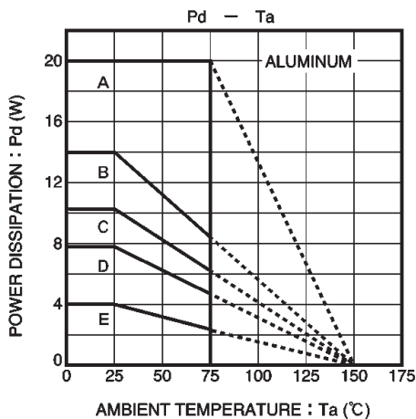
Fig. 10 Power dissipation curves (BA5415A)
