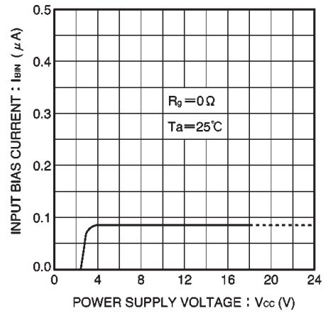
Fig. 18 Input bias current vs. power supply voltage
