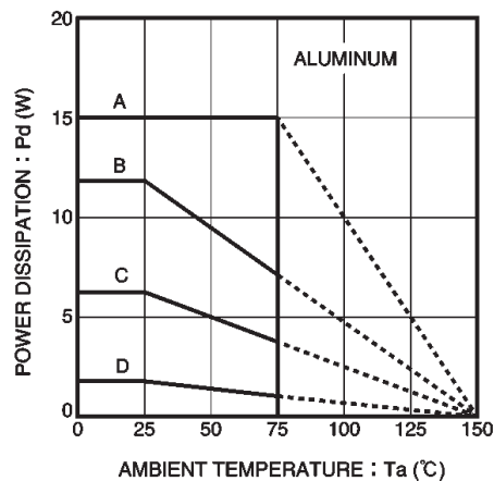
Fig. 11 Power dissipation curves (BA5416)
