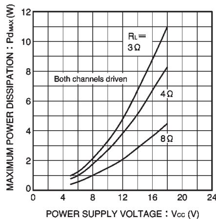
Fig. 29 Maximum power dissipation vs. power supply voltage
