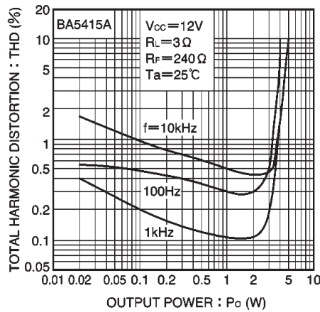
Fig. 14 Total harmonic distortion vs. output power (BA5415A)
