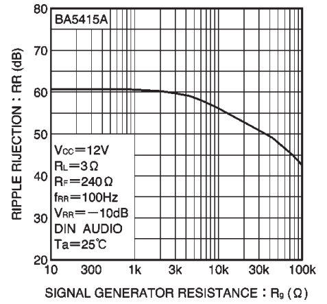
Fig. 27 Ripple rejection vs. signal source resistance (BA5415A)
