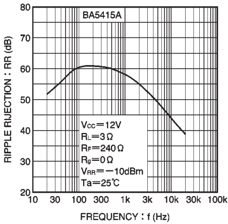
Fig. 25 Ripple rejection vs. frequency (BA5415A)
