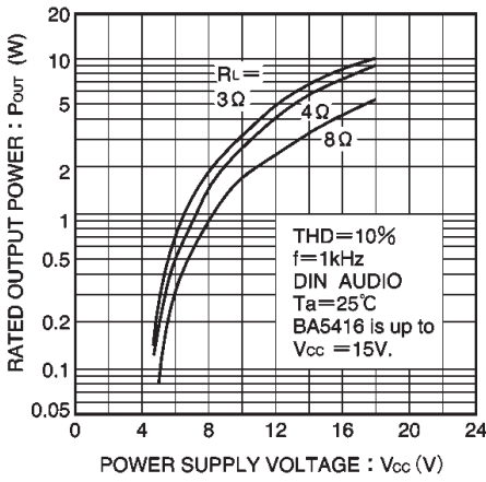
Fig. 16 Rated output voltage vs. power supply voltage
