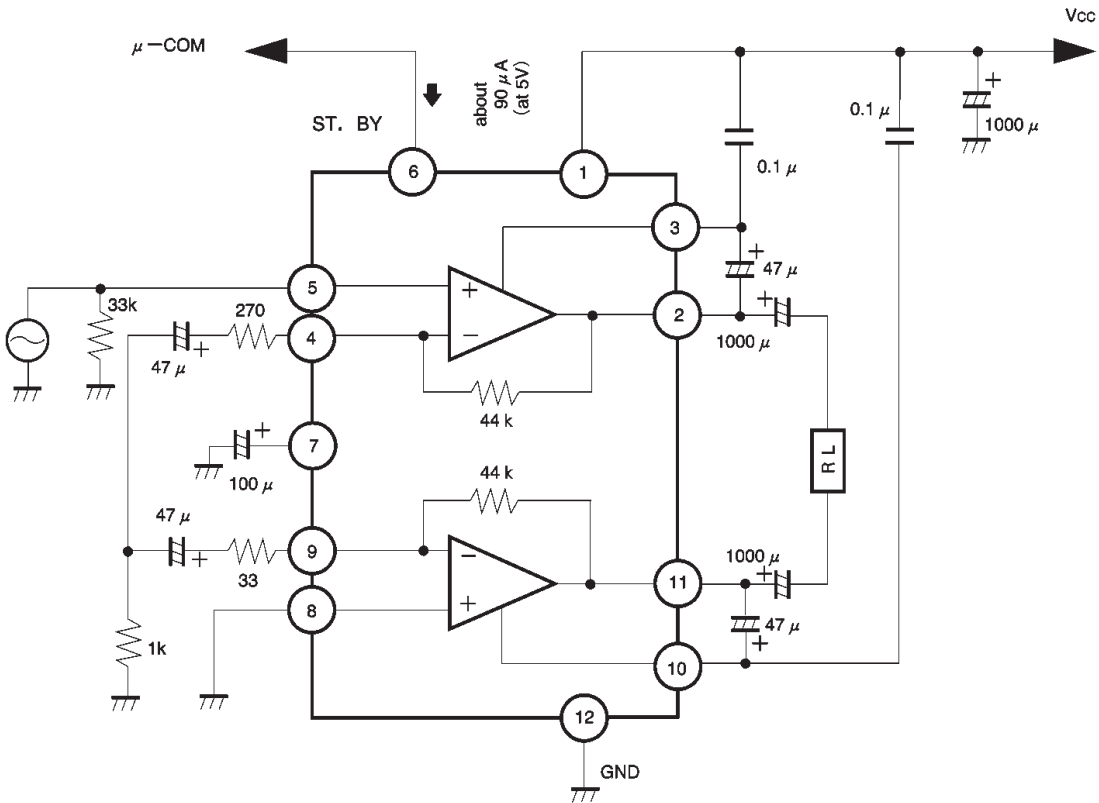
Fig. 3 BTL Application circuit example
