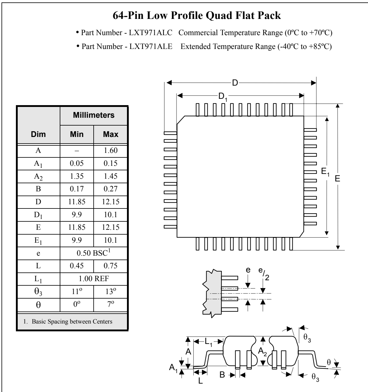
Figure 44. LXT971A LQFP Package Specifications
