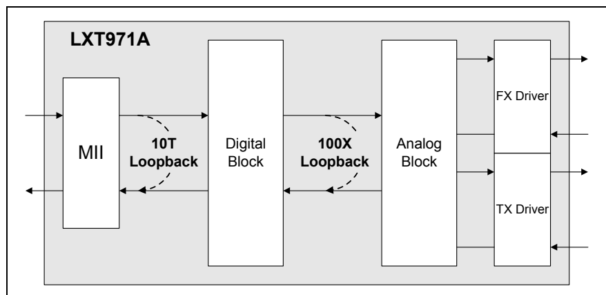
Figure 13. Loopback Paths
