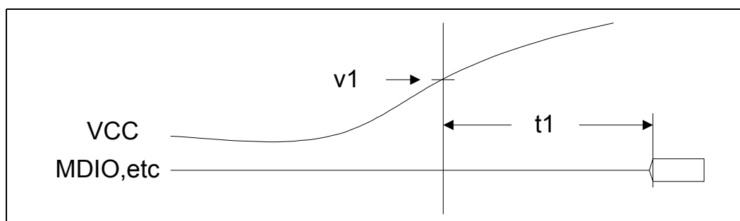
Figure 40. Power-Up Timing
