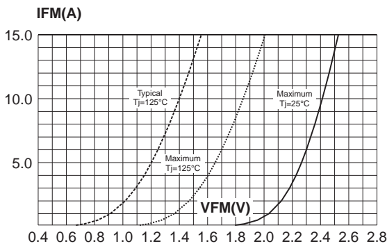
Fig. 3: Forward voltage drop versus forward current
