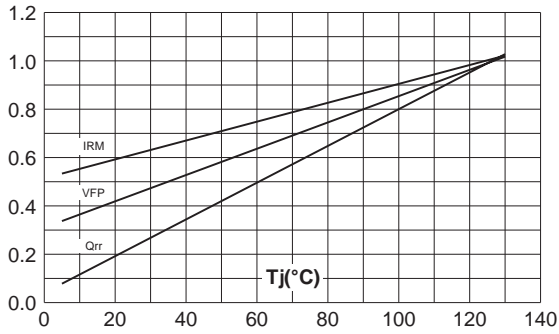
Fig. 9: Dynamic parameters versus junction temperature
