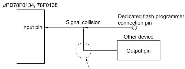
Figure 27-15. Signal Collision (Input Pin of Serial Interface)
