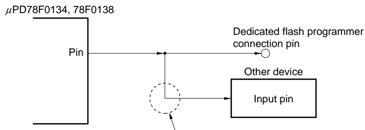
Figure 27-16. Malfunction of Other Device
