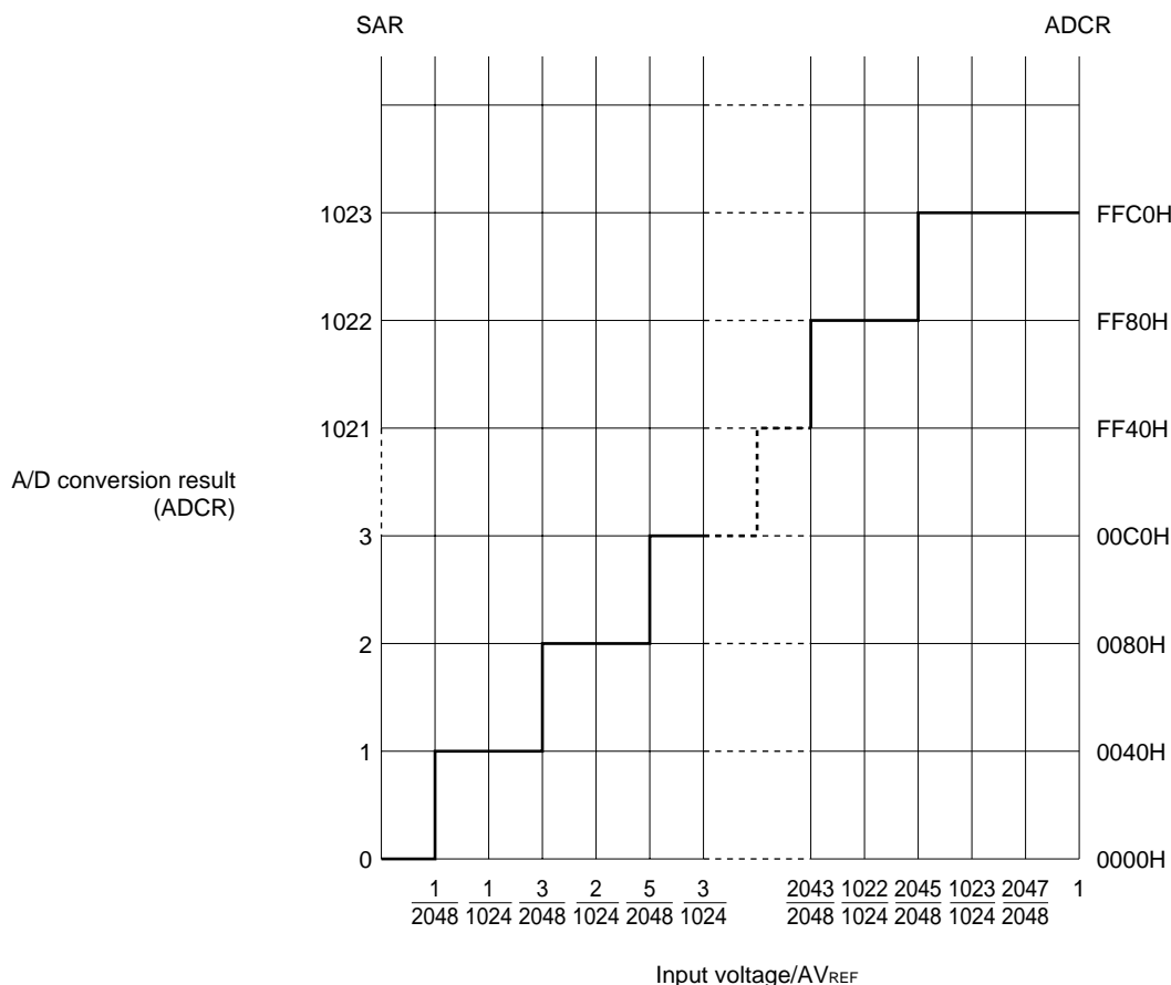
★ Figure 12-9. Relationship Between Analog Input Voltage and A/D Conversion Result
