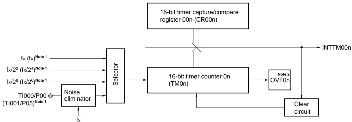
Figure 6-16. Interval Timer Configuration Diagram
