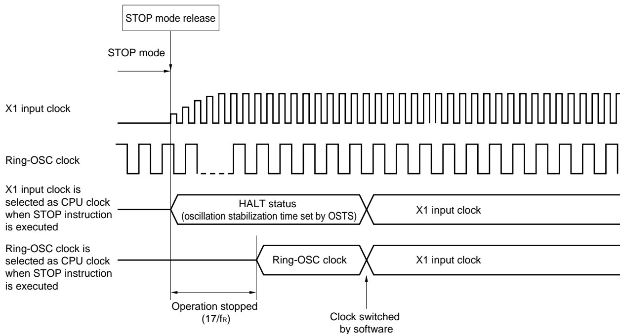
Figure 19-5. Operation Timing When STOP Mode Is Released
