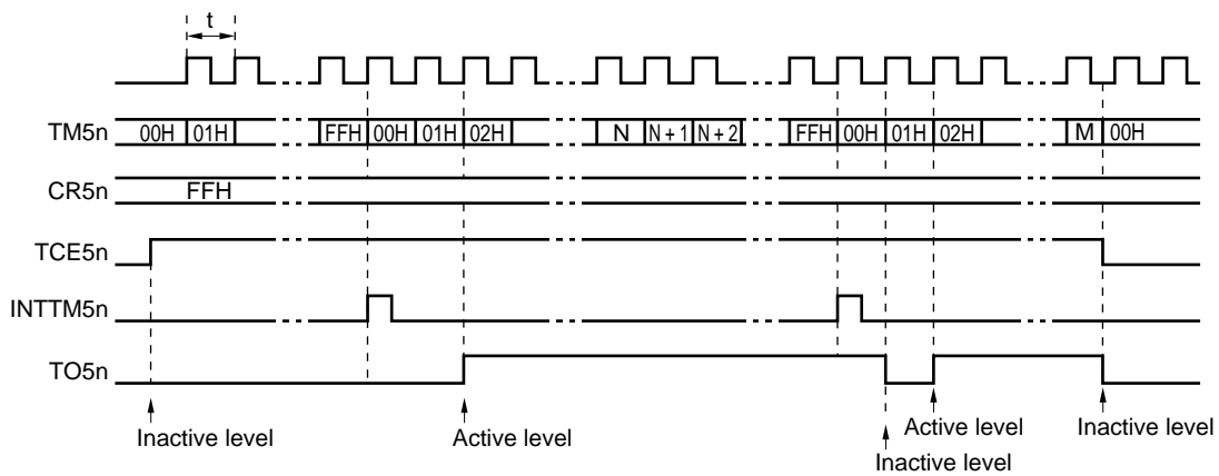
(c) CR5n = FFH
