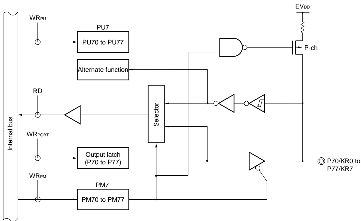
Figure 4-17. Block Diagram of P70 to P77
