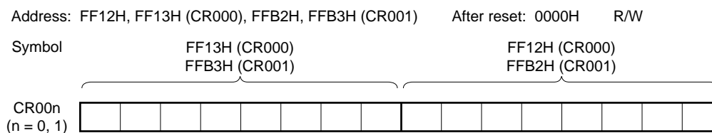
Figure 6-4. Format of 16-Bit Timer Capture/Compare Register 00n (CR00n)
