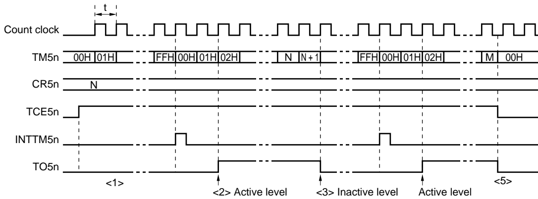
(b) CR5n = 00H
