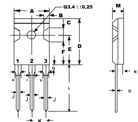
TO-247 (3P)
