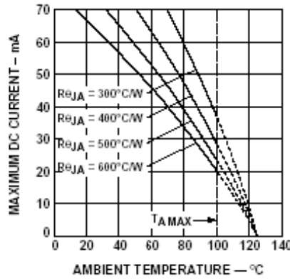
Figure 3.4A. Maximum DC Forward Current versus Ambient Temperature for HPWA-xx00 LED Emitter with Different System Thermal Resistances.
