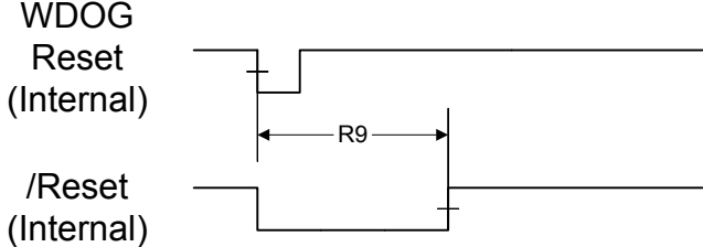
Figure 20-15. Watchdog Reset Timing
