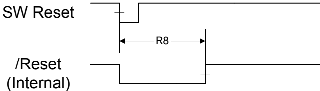
Figure 20-15. Watchdog Reset Timing
