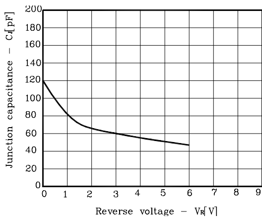
Fig. 5 Capacitance vs Reverse voltage
