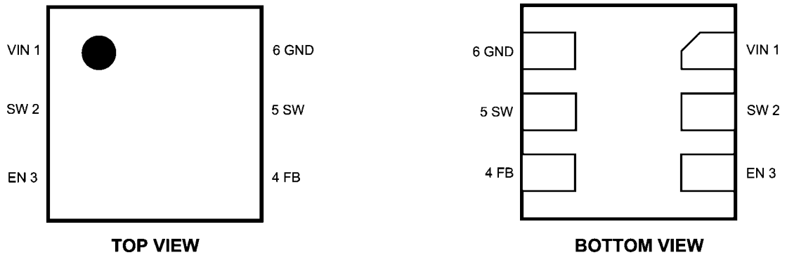
FIGURE 4. 6 Pin LLP Package
