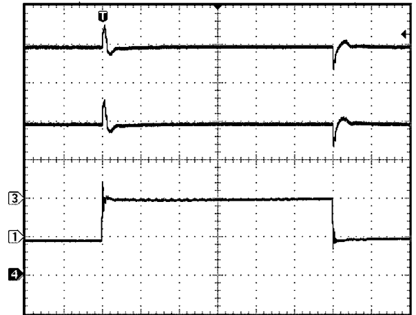
Line Step (LED Mode) (2 x 5 LEDs, 20mA per String, C OUT = 1µF, V IN from 3V to 3.6V)
