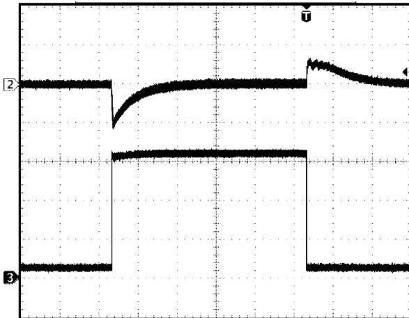
Load Step (OLED Mode) (V OUT = 18V, C OUT = 2.2µF)
