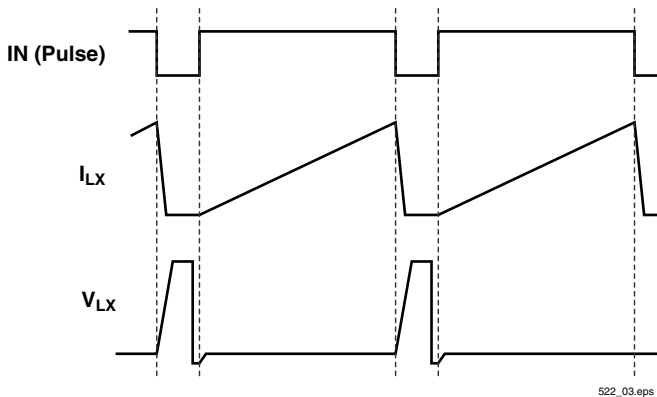
Figure 1. Driver Waveforms
