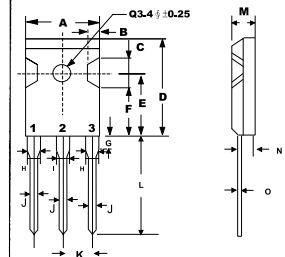
TO-247 (3P)
