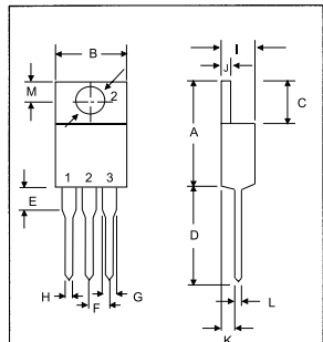
TO-220AB
