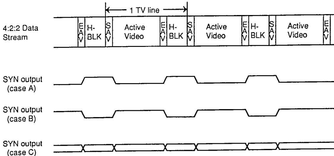
Fig. 10-1. SYNC output in 4:2:2 case (not to scale)
