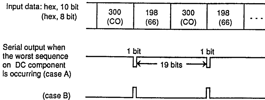
Fig. 10-3. Particular data words for checking equalization and AGC time-constant
