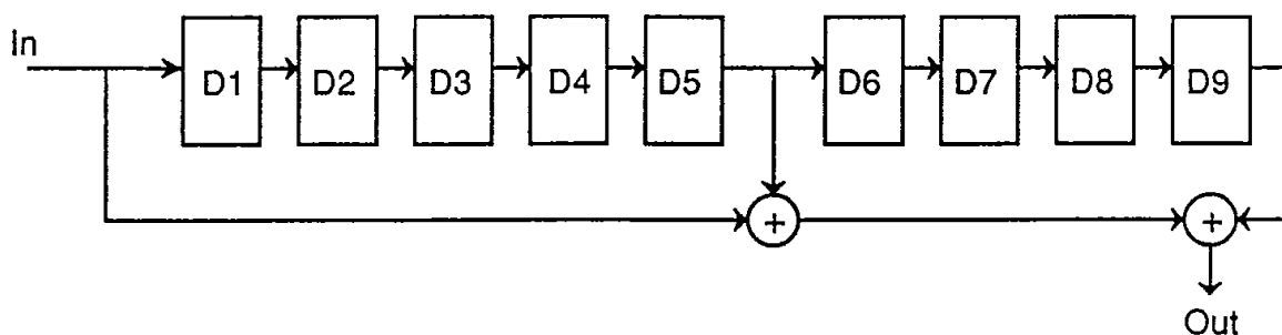
Fig. 9-9 (a). X^9 + X^4 + 1 descrambler
