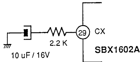
Fig. 9-3. AGC time-constant
