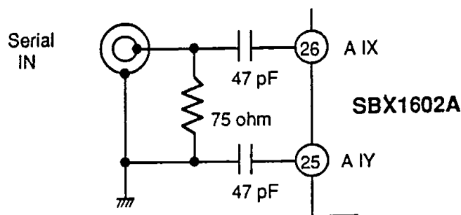
Fig. 9-1 (a). Equalizer Input circuit with capacitor coupling
