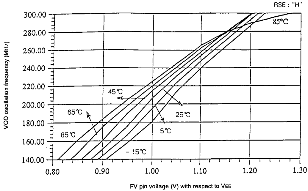
Fig. 11-1. VCO oscillation frequency vs. control voltage at high rate
