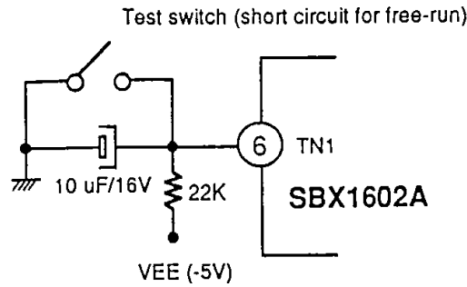
Fig. 9-6. Transient absorber time-constant
