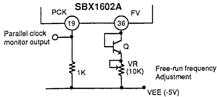
Fig. 9-7. Compensation on VCO temperature characteristics
