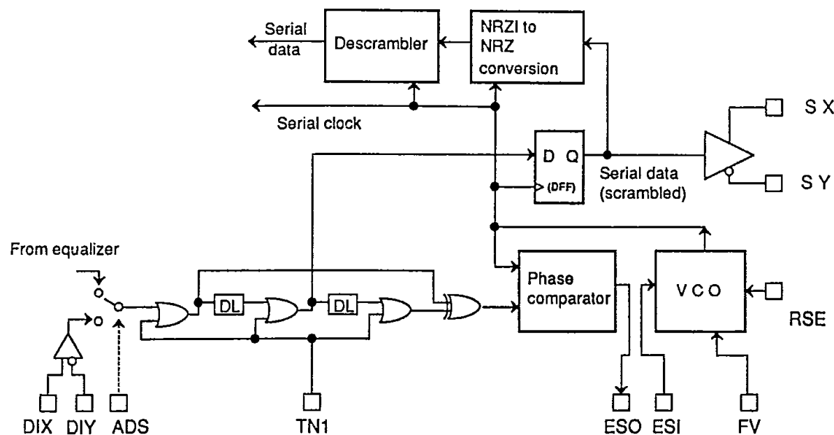
Fig. 9-5. Serial data input and PLL block
