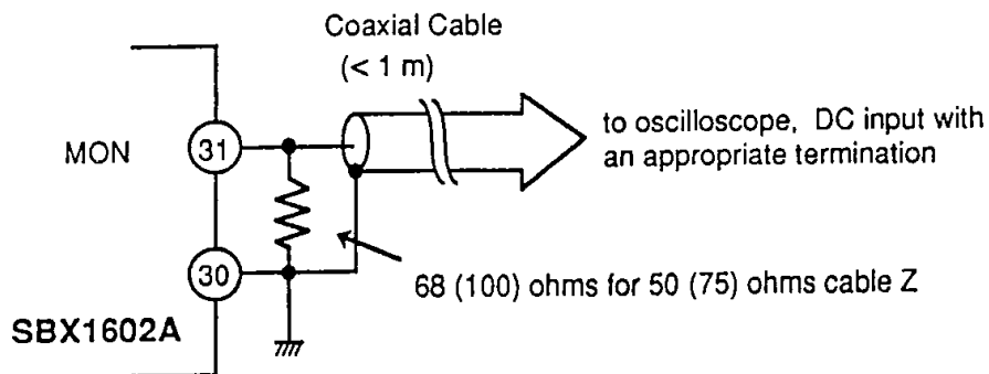
Fig. 9-4. Eye monitoring
