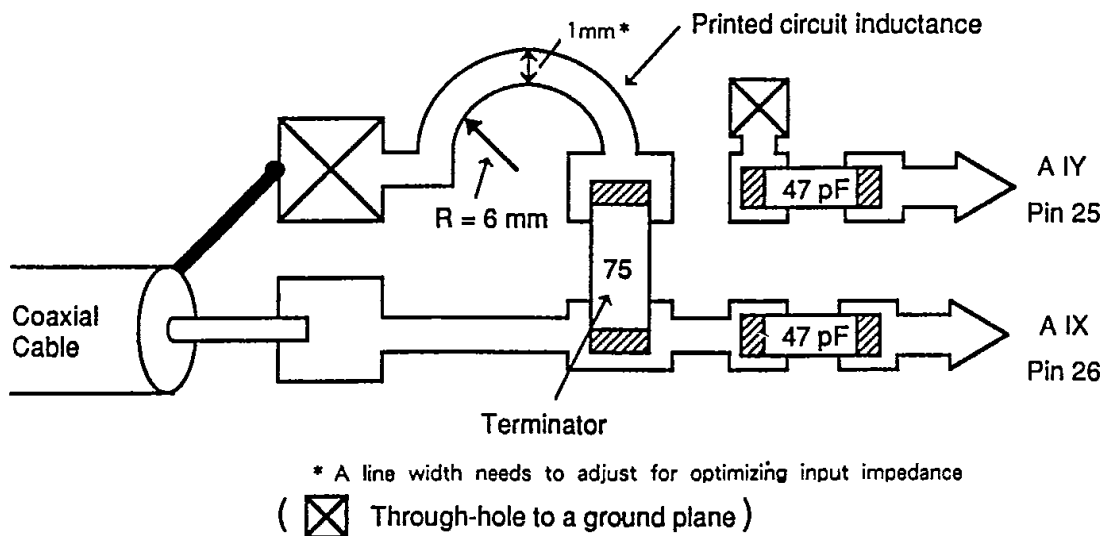
Fig. 9-2. An example of technique to improve the return-loss figure for the capacitor coupling input case.
