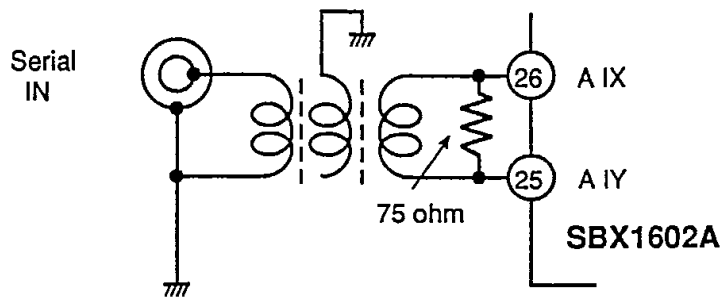
Fig. 9-1 (b). Equalizer input circuit with transformer coupling
