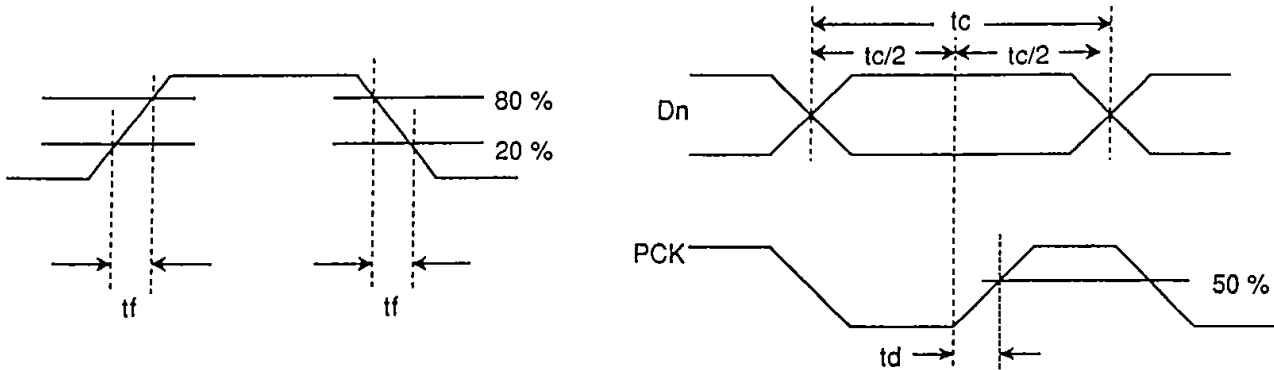
Fig. 8-1. Definition of t_r, t_f, t_c, t_d
