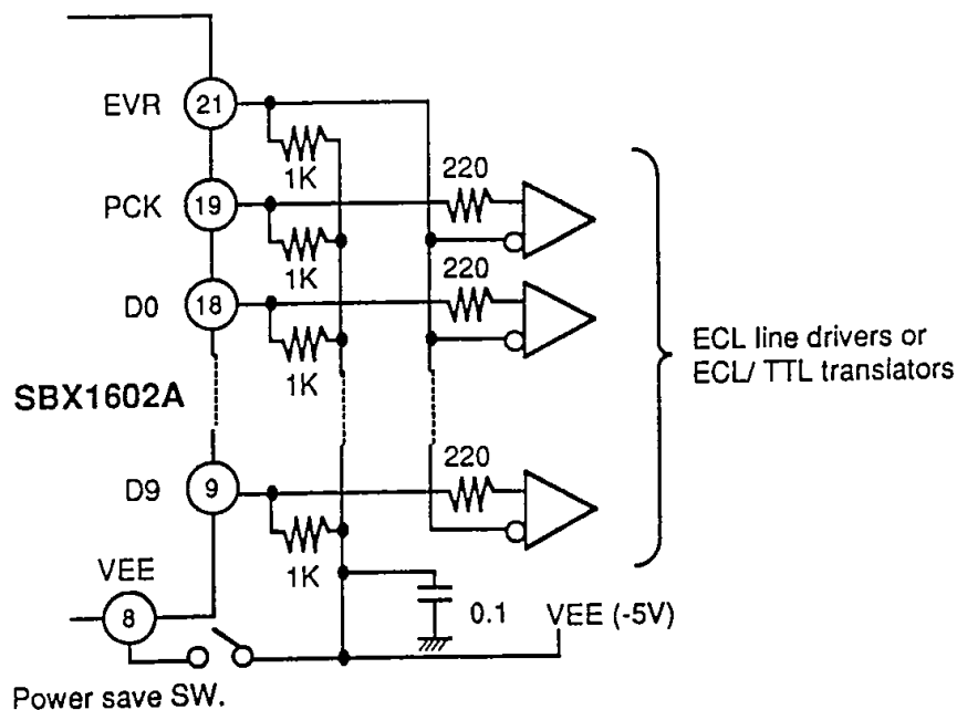
Fig. 9-10. A suggested parallel clock/data output circuit
