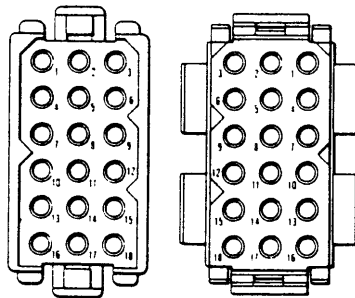
Plug
