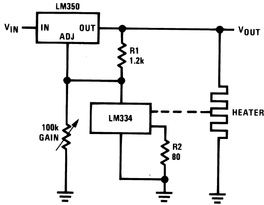
Temperature Controller
