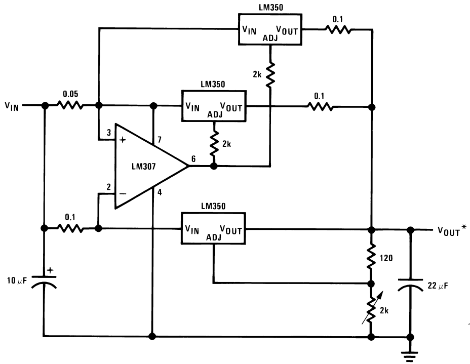
10A Regulator
