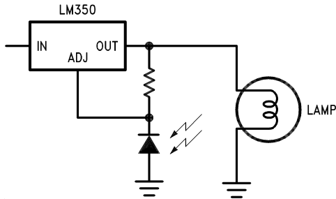
Light Controller
