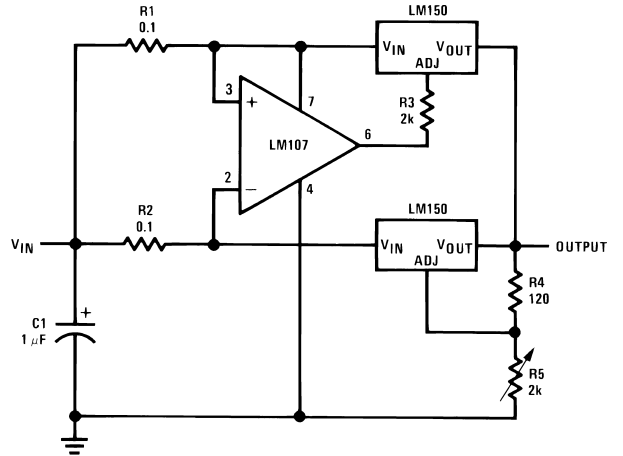
6A Regulator
