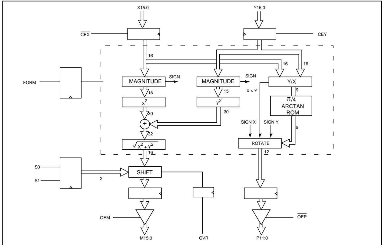
Fig.2 Block diagram
