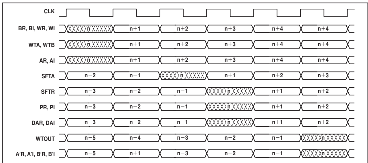
Fig. 6 Butterfly data and control signals
