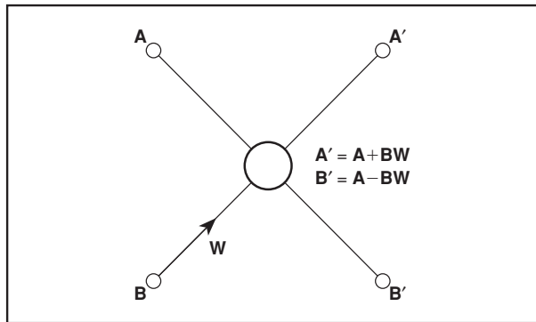
Fig. 5 Butterfly operation
