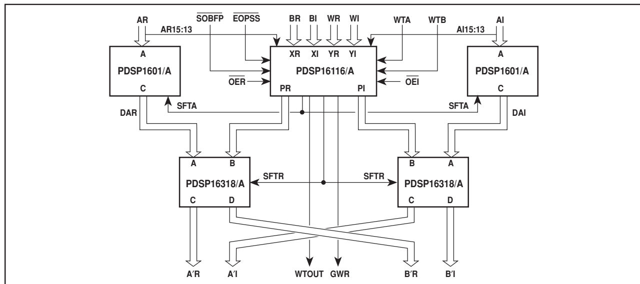
Fig. 4 FFT butterfly processor
