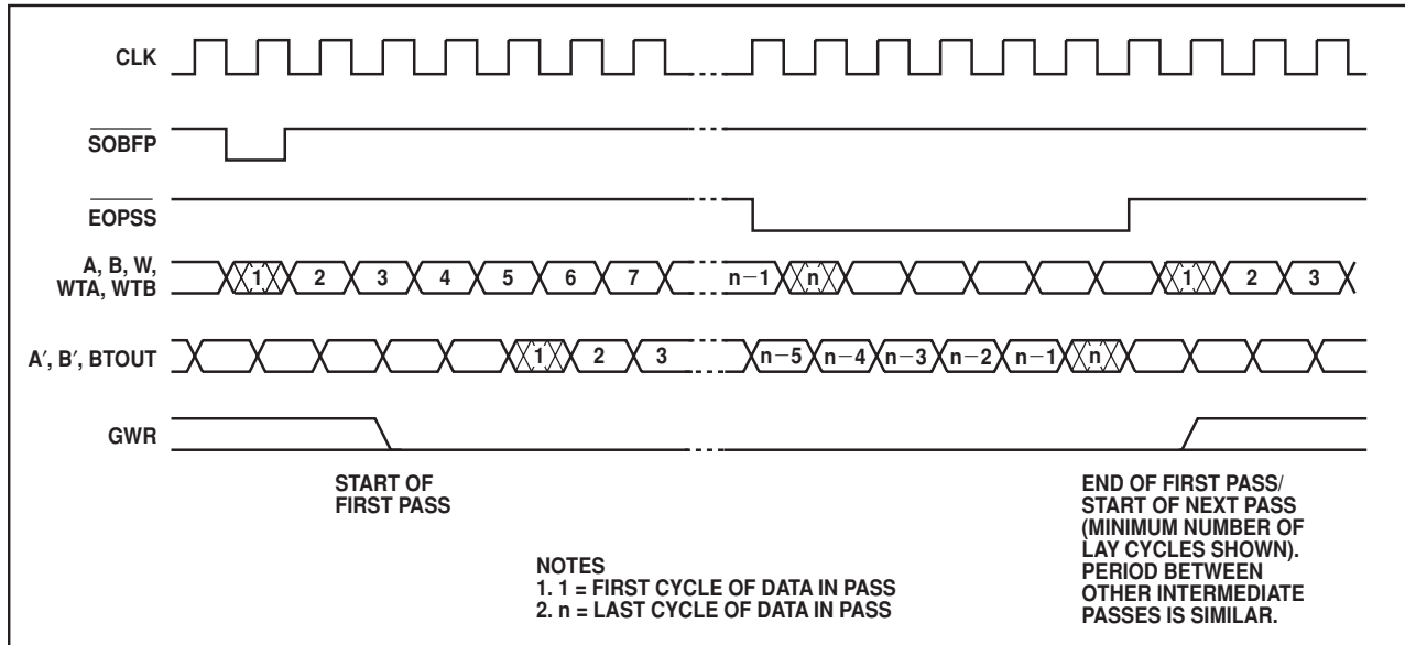
Fig. 7 Use of the BFP control signals
