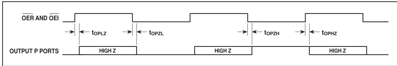
Fig. 10 Output tristate timing
