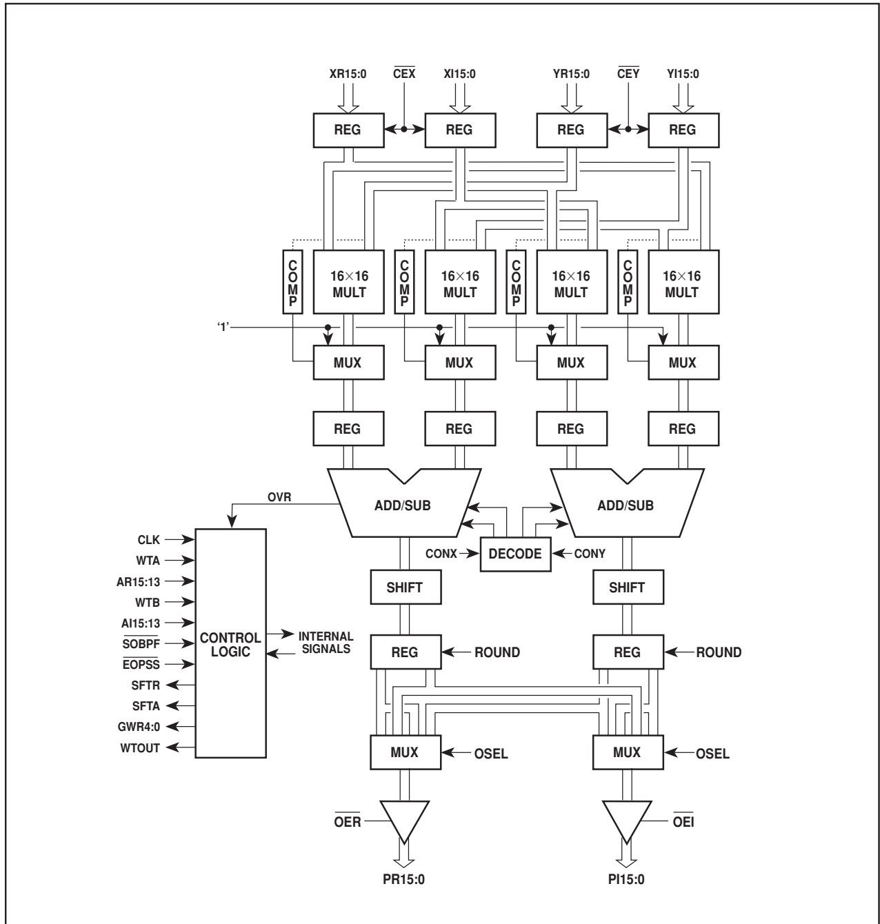
Fig. 2 PDSP16116 Block diagram
