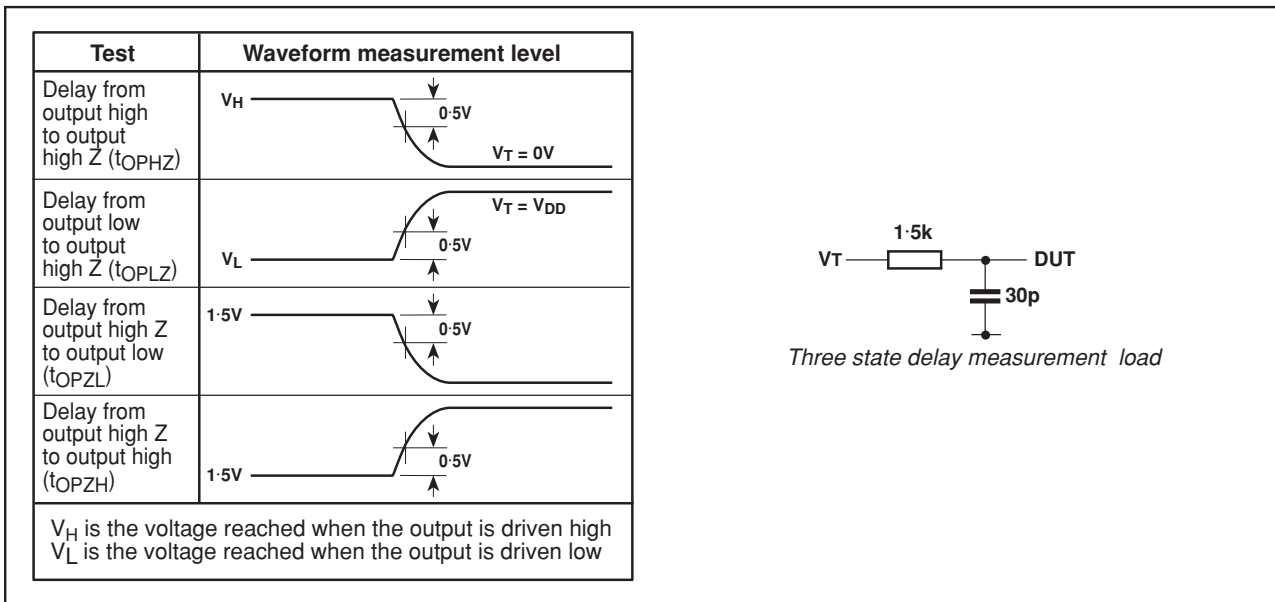
Fig. 11 Three state delay measurement
