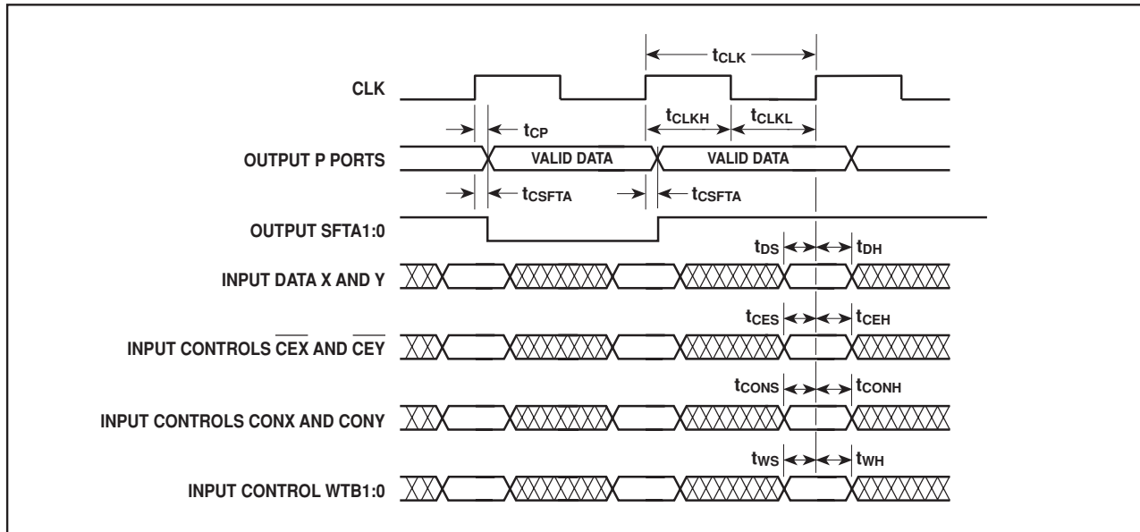
Fig. 9 Normal mode timing
