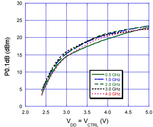
P0.1dB
