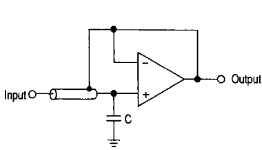
Figure 17. Cable Bootstrapping and Input Shields
