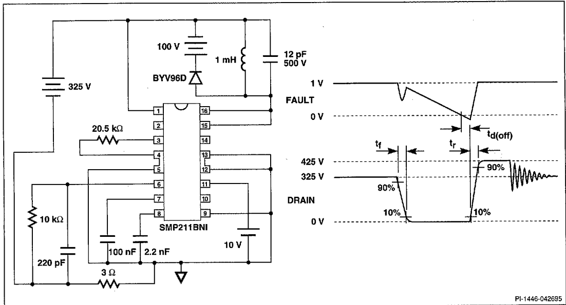
Figure 8. Current Limit Delay/Switching Time Test Circuit.
