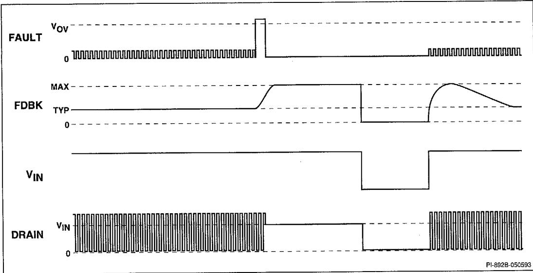
Figure 5. Typical Waveforms for Overvoltage Shutdown.
