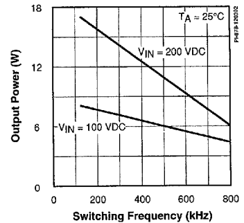
OUTPUT POWER vs. FREQUENCY
