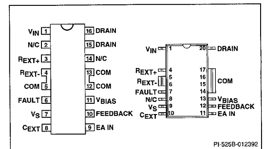
Figure 2. Pin Configuration
