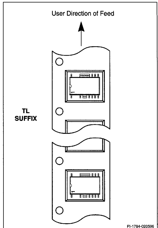
Figure 1. Part Orientation and Ordering Suffix.
