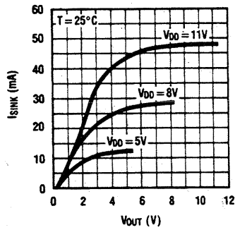
FIGURE 1. I_{SINK} vs V_{OUT}
