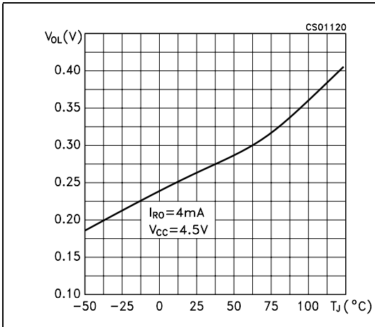
Figure 16. Receiver low level output voltage vs. temperature
