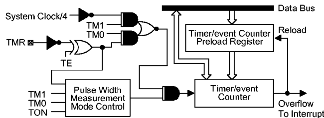
Timer/event counter
