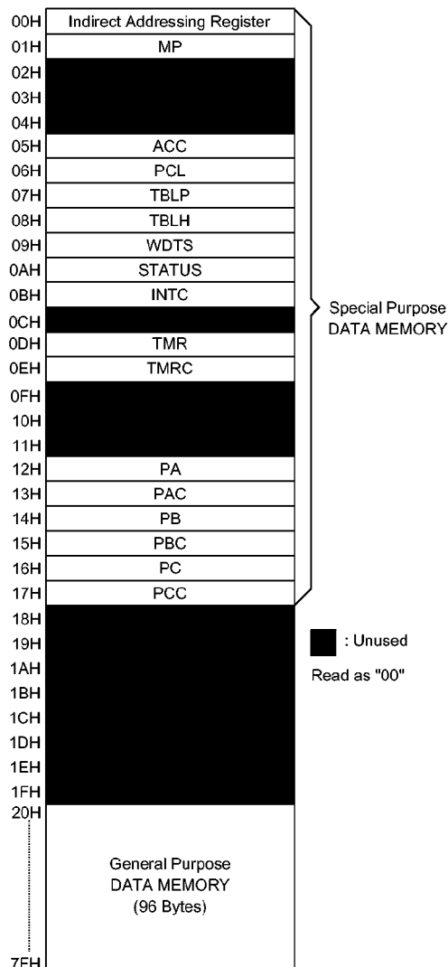
RAM mapping
