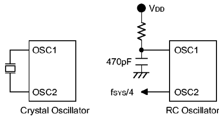
System oscillator
