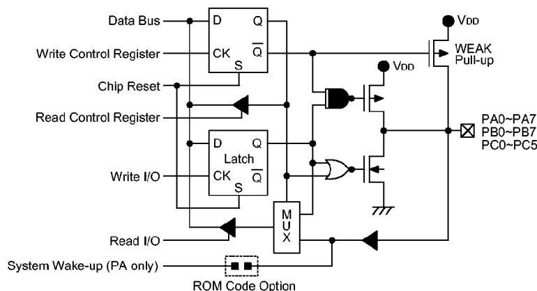
Input/output ports
