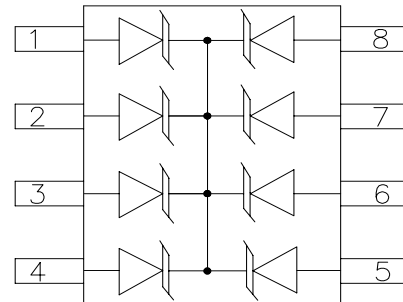
Connection Diagram
