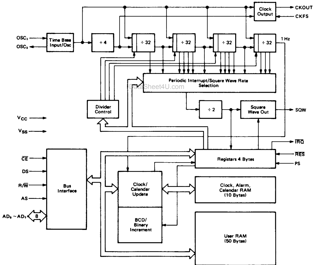
Figure 10 Block Diagram
