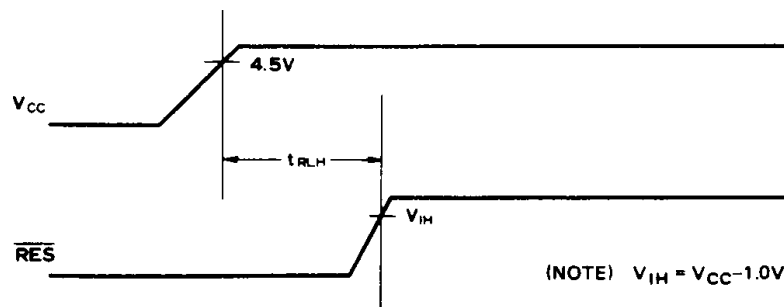
Figure 7 \overline{RES} Release Delay
