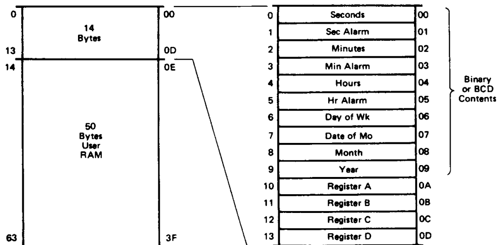
Figure 14 Address Map
