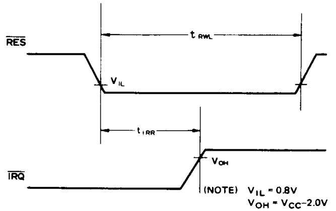
Figure 5 \overline{IRQ} Release Delay (from \overline{RES} )
