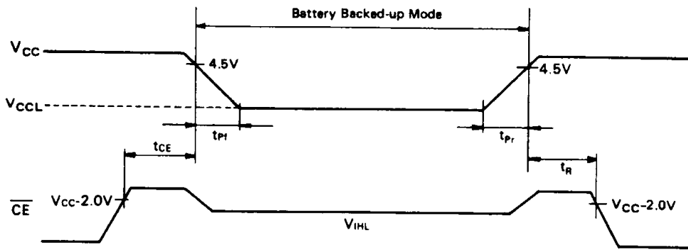
Figure 9 Battery Backed-up Timing
