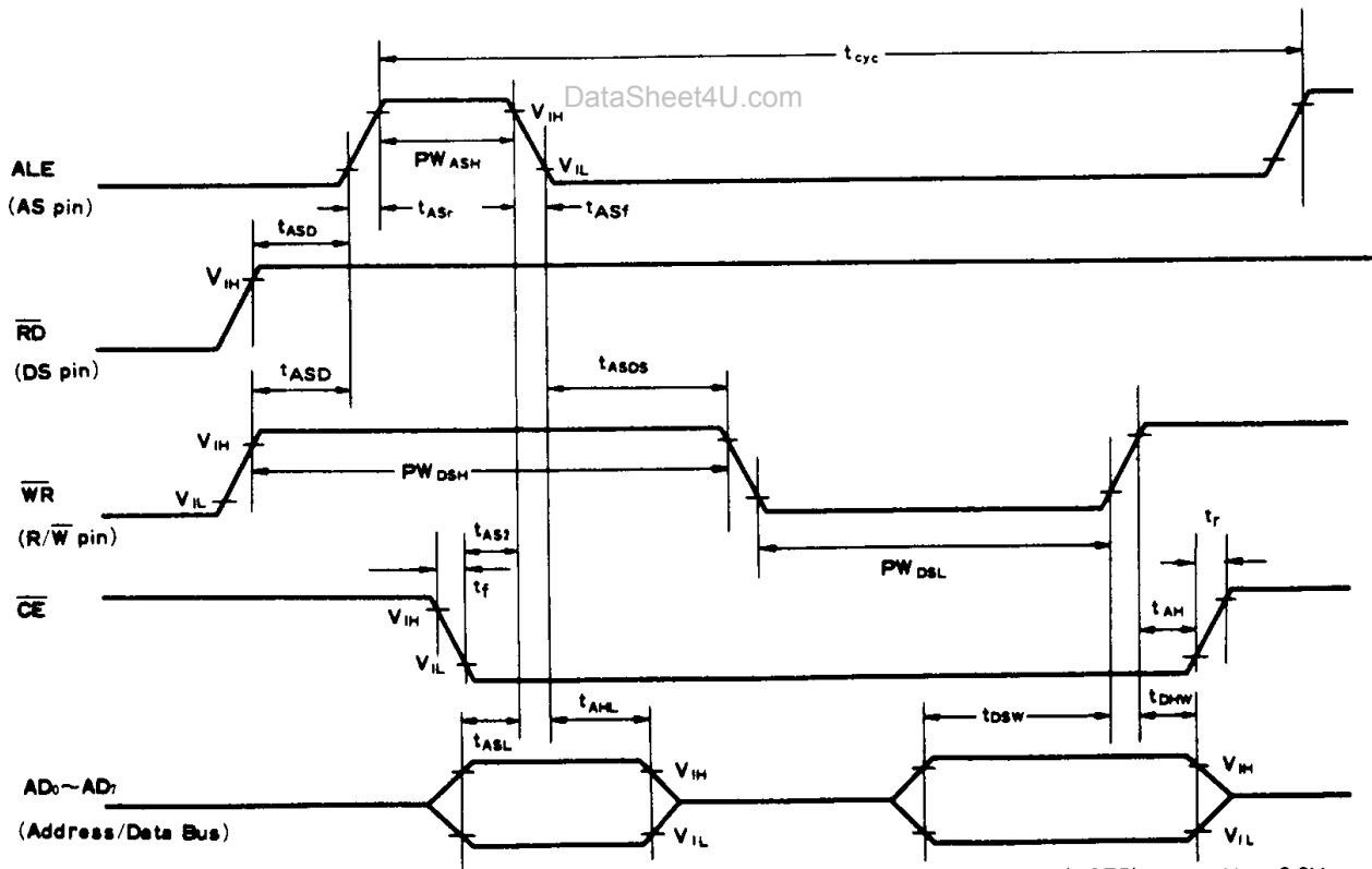
Figure 3 Write Timing (8085 Family)
