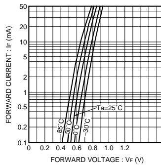
Fig.2 Forward current vs. forward voltage (P Type)
