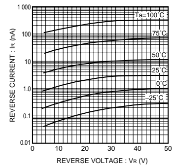
Fig.3 Reverse current vs. reverse voltage (P Type)
