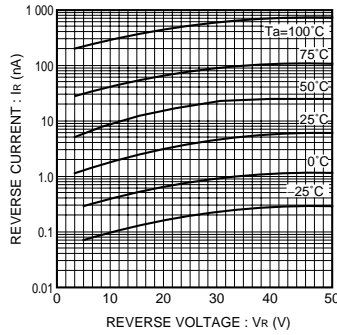
Fig.5 Reverse current vs. reverse voltage (N Type)
