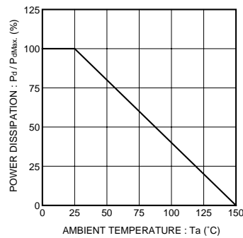
Fig.1 Power reduction curve
