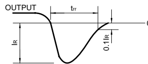
Fig.8 Reverse recovery time ( t_{rr} ) measurement circuit
