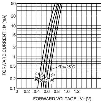
Fig.4 Forward current vs. forward voltage (N Type)
