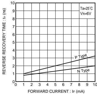
Fig.7 Reverse recovery time vs. forward current
