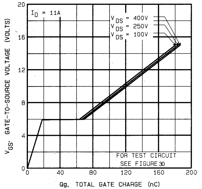
Fig 23. Typical Gate Charge Vs. Gate-to-Source Voltage
