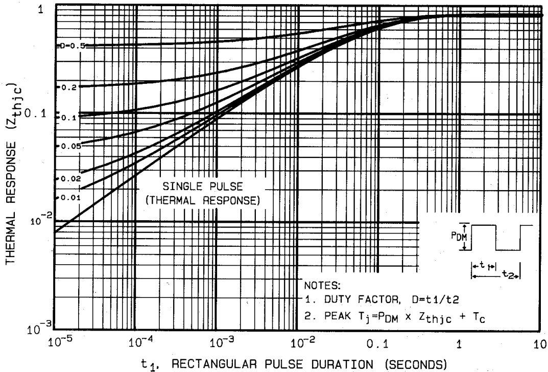
Fig 28. Maximum Effective Transient Thermal Impedance, Junction-to-Case
