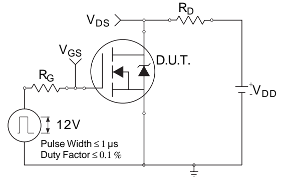
Fig 27a. Switching Time Test Circuit
