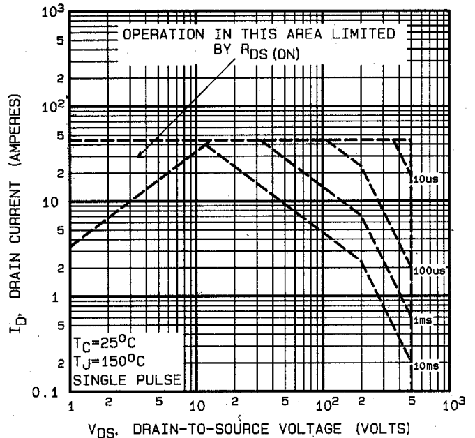
Fig 25. Maximum Safe Operating Area
