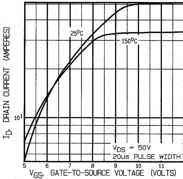
Fig 20. Typical Transfer Characteristics
