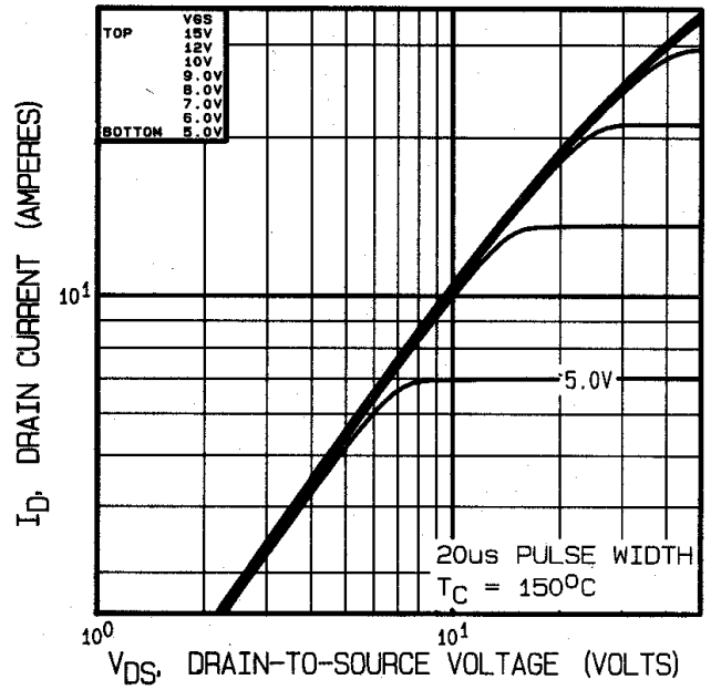
Fig 19. Typical Output Characteristics
