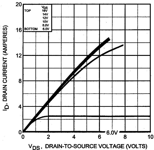
Fig 12. Typical Output Characteristics Post-Irradiation 300K Rads (Si)
