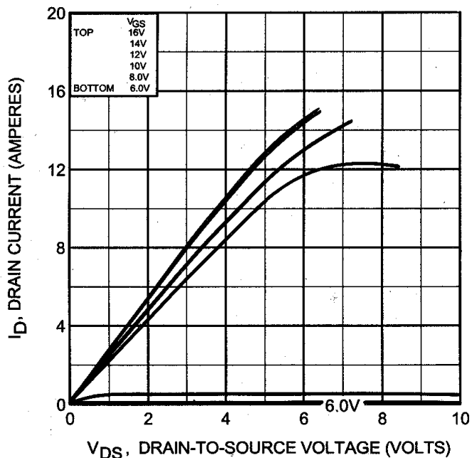
Fig 10. Typical Output Characteristics Pre-Irradiation
