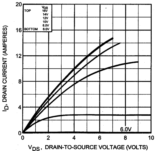
Fig 13. Typical Output Characteristics Post-Irradiation 1 Mega Rads (Si)
