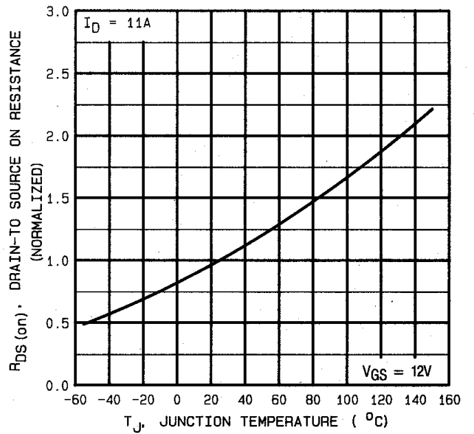
Fig 21. Normalized On-Resistance Vs. Temperature
