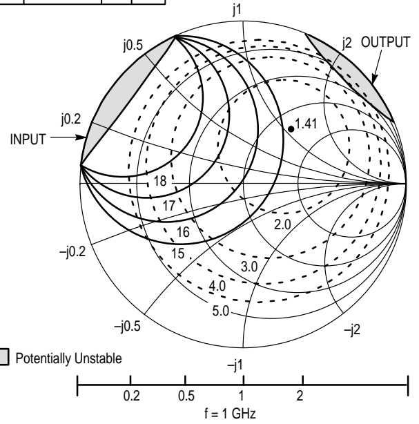
Figure 22. MRF949T1 Series Constant Gain and Noise Figure Contours
