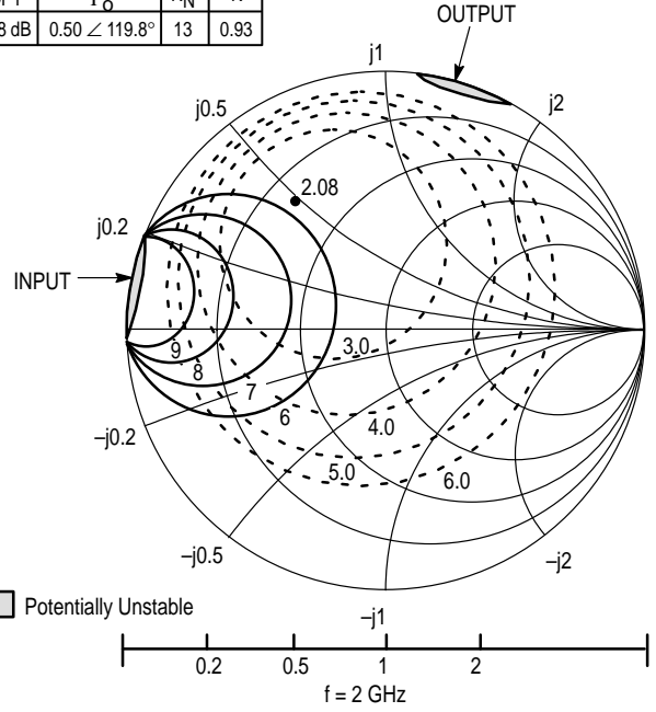
Figure 20. MRF949T1 Series Constant Gain and Noise Figure Contours
