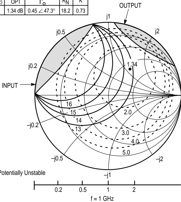
Figure 21. MRF949T1 Series Constant Gain and Noise Figure Contours
