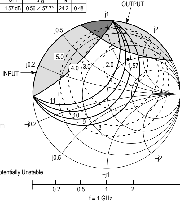
Figure 19. MRF949T1 Series Constant Gain and Noise Figure Contours
