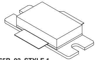
CASE 465B-03, STYLE 1 NI-880 MRF5S21130
