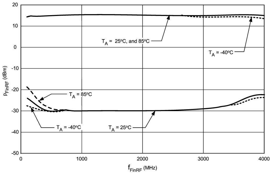
RF PLL Fin Sensitivity V_{CC} = 3.0 V , RF_P = 16
