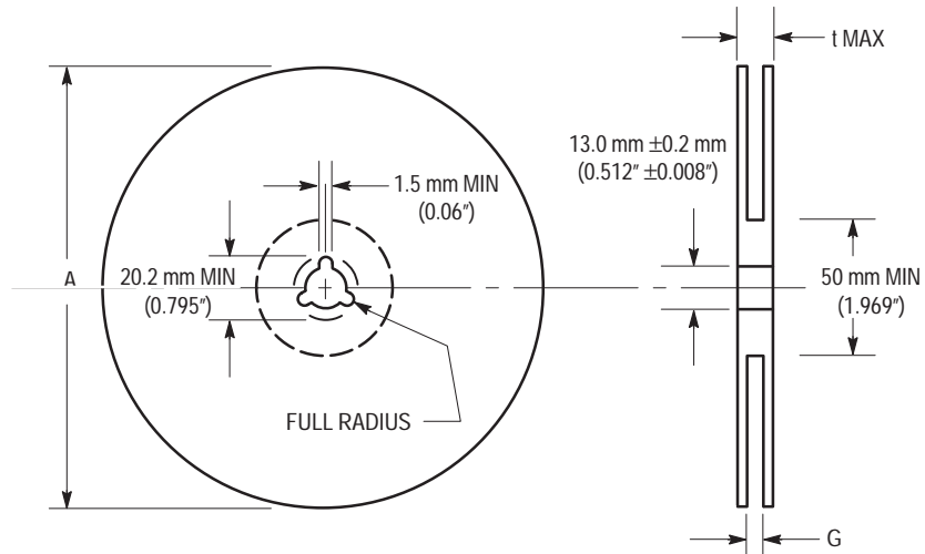
Figure 5. Reel Dimensions
