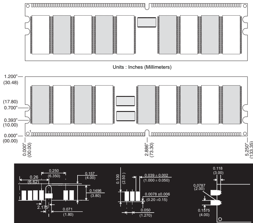
Figure 1: KVR400X72R8C3A/512 184-Pin DIMM
