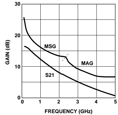
Figure 19. AT-32011 Gains vs. Frequency at V_{CE} = 2.7 V, I_C = 2 mA .
