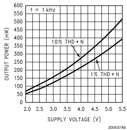
Output Power vs Supply Voltage, 32Ω
