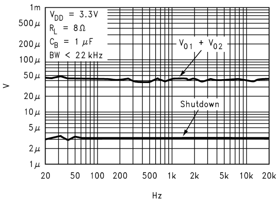
Noise Floor
